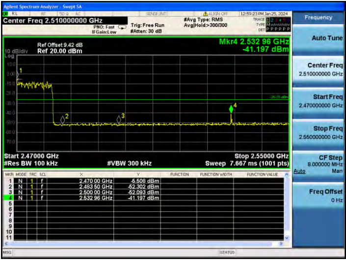
3DH5_Ant1_High_Hop_2480
