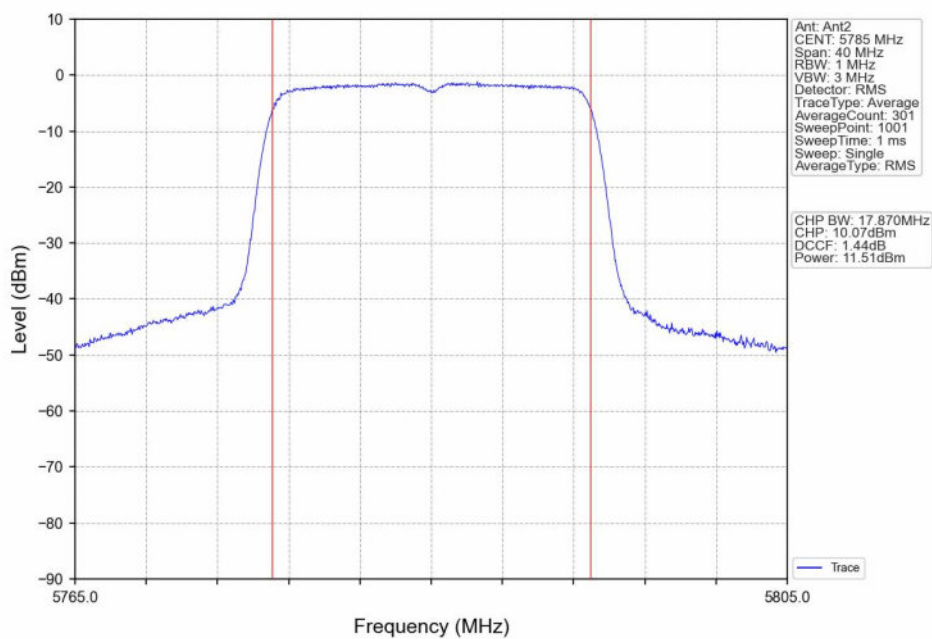
802.11n(HT20)_MCH_5785MHz_Ant2_NTNV
