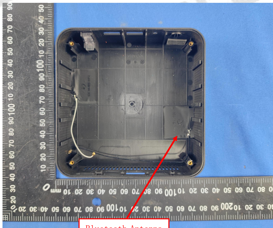
Bluetooth Antenna
