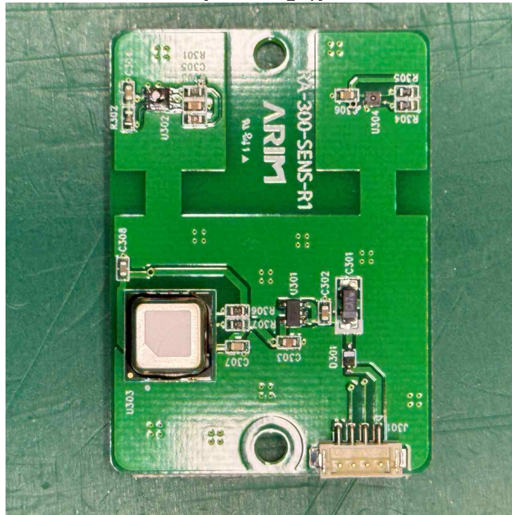
[SENS Board_Top]
