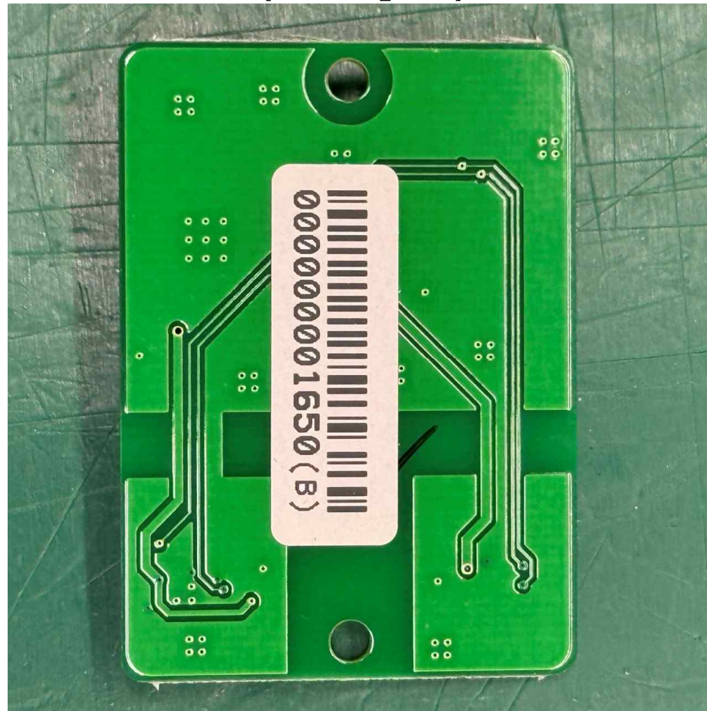
[SENS Board_Bottom]
