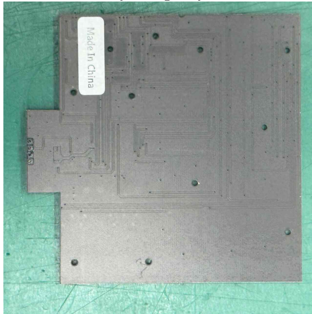
[LED Board_Bottom]
