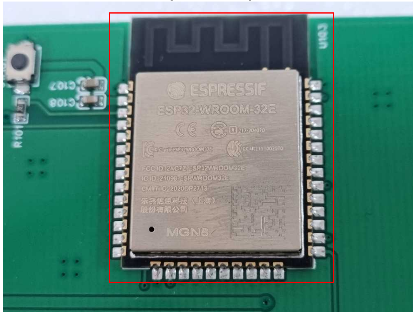
[Certificated module]
