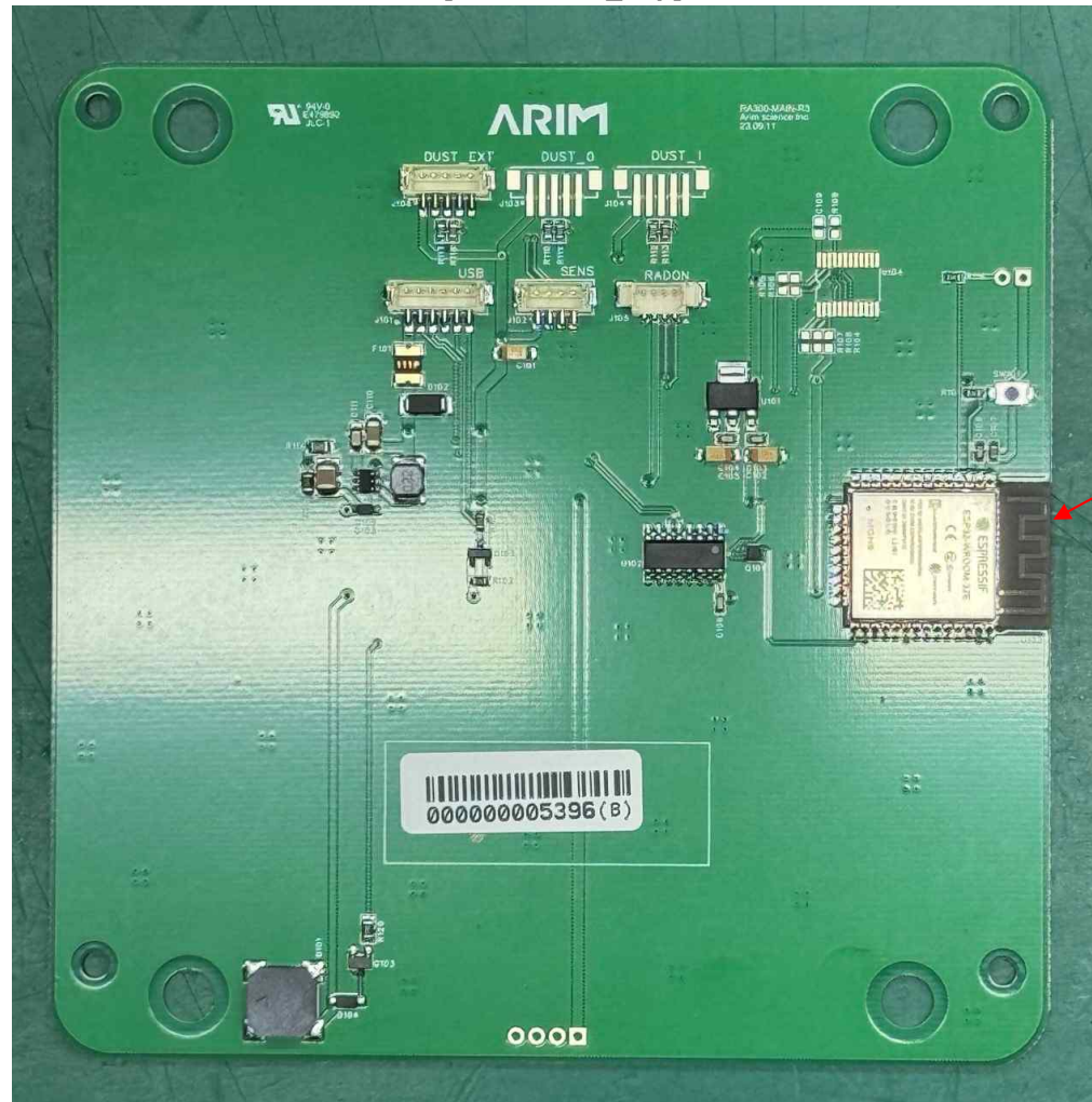
[Main board_Top]
