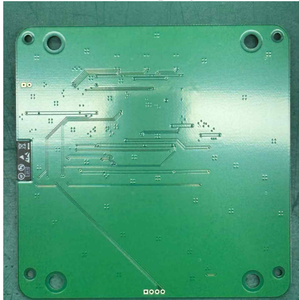
[Main board_Bottom]
