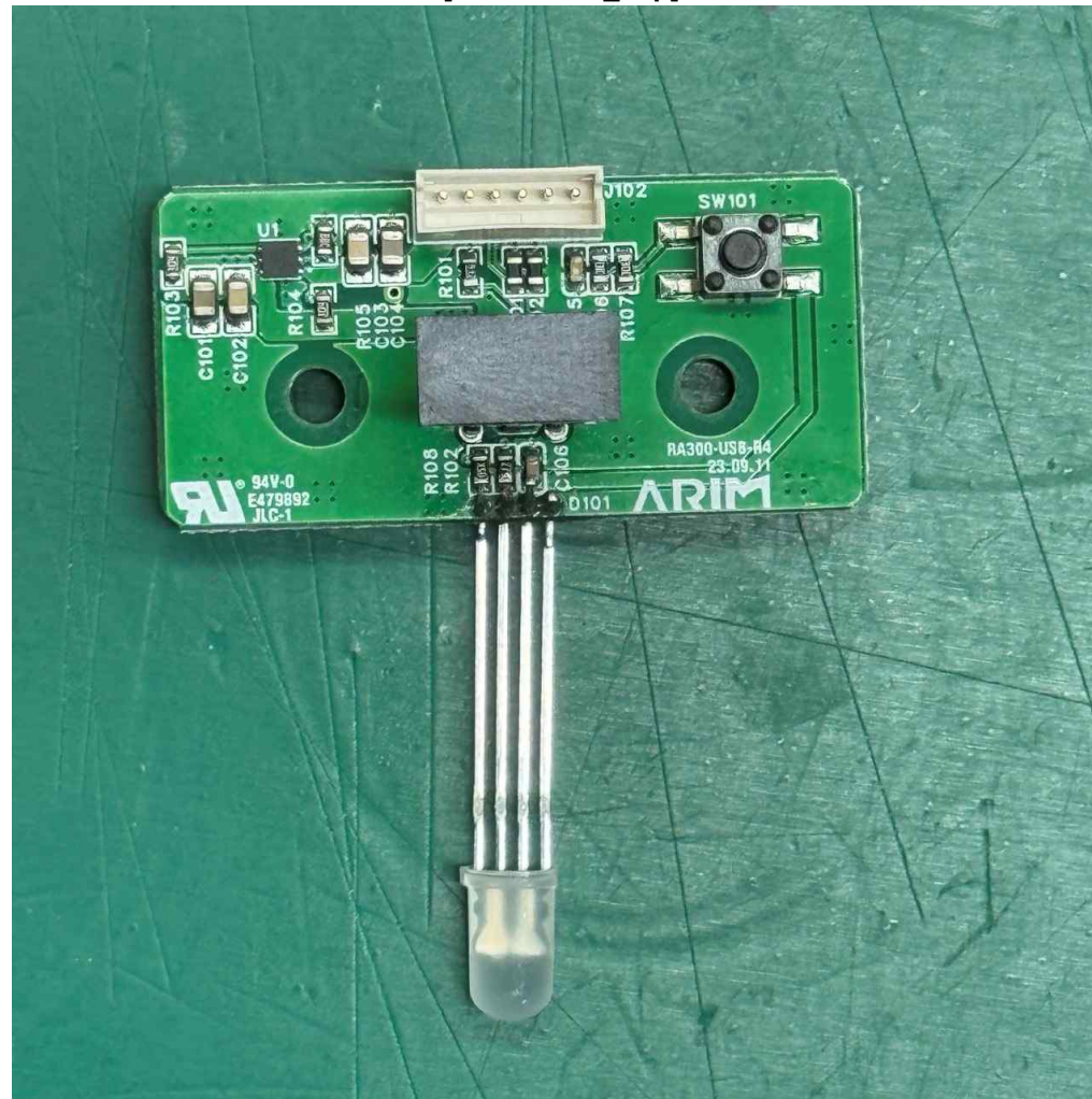
[USB Board_Top]
