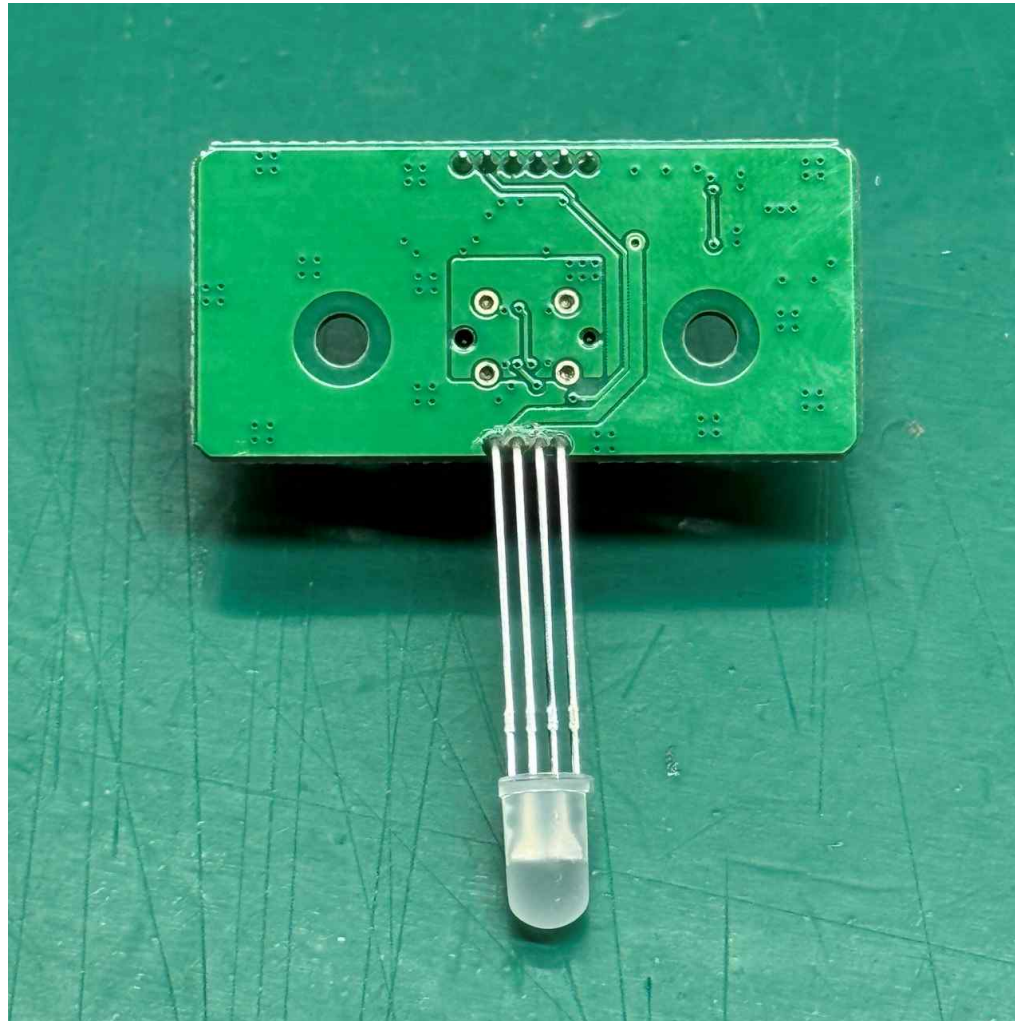
[USB Board_Bottom]
