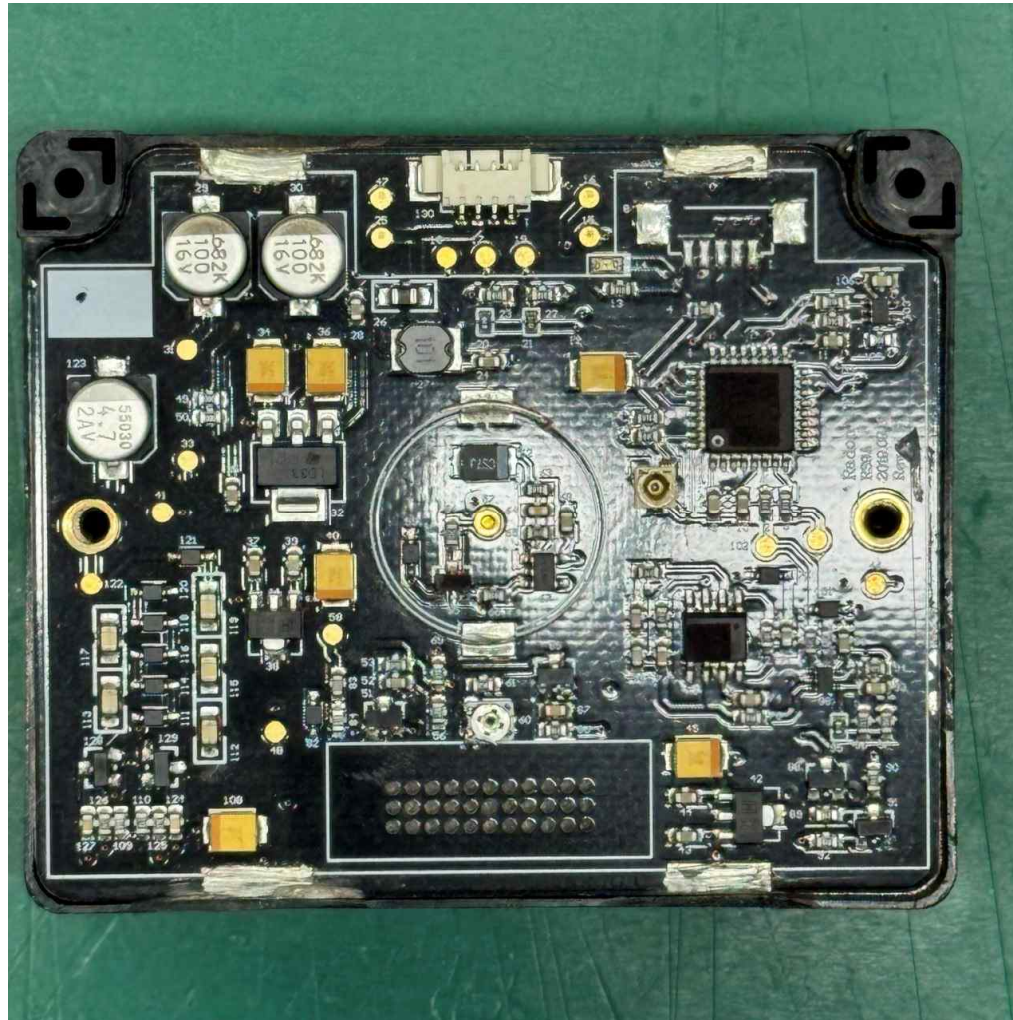
[RS9A Board_Bottom]
