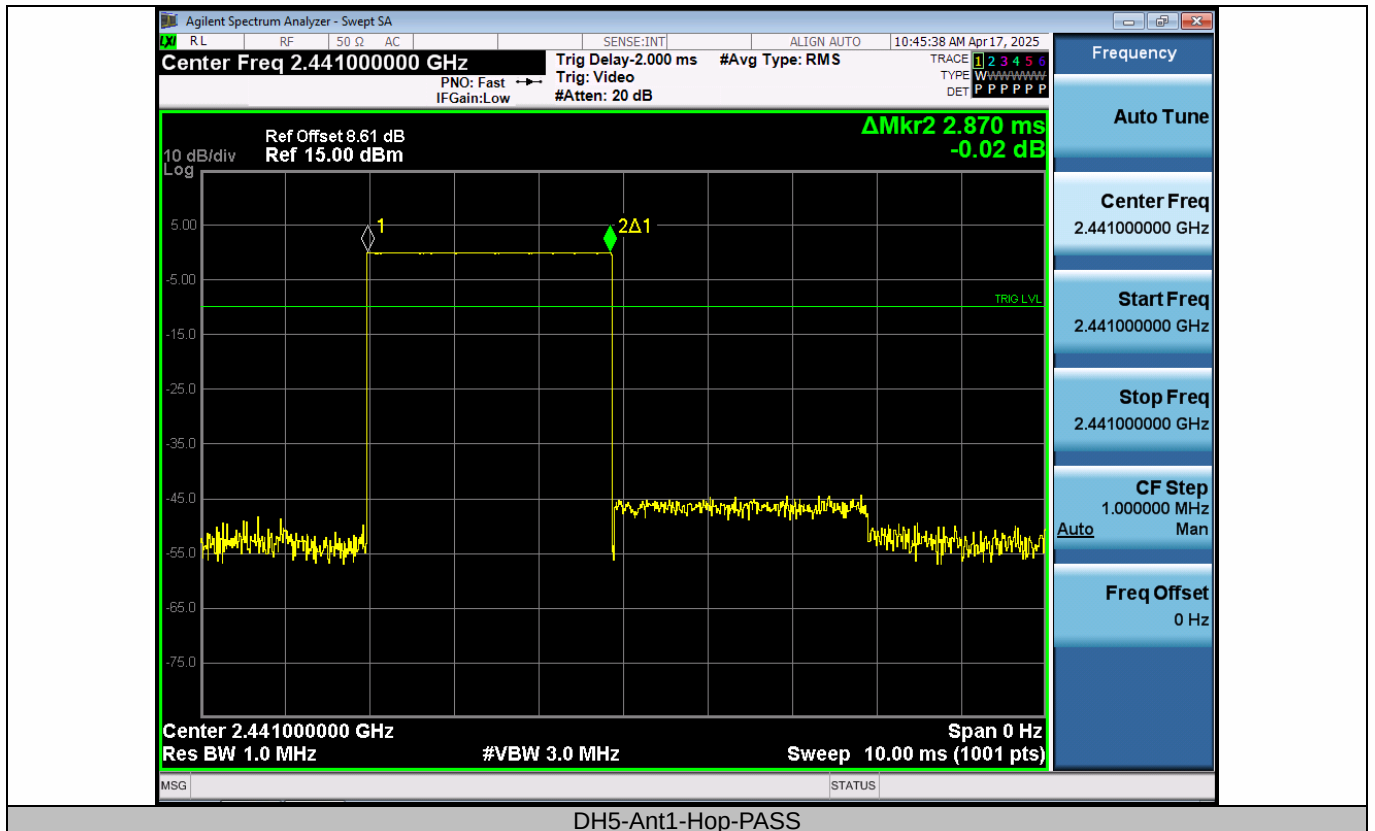
DH5-Ant1-Hop-PASS
