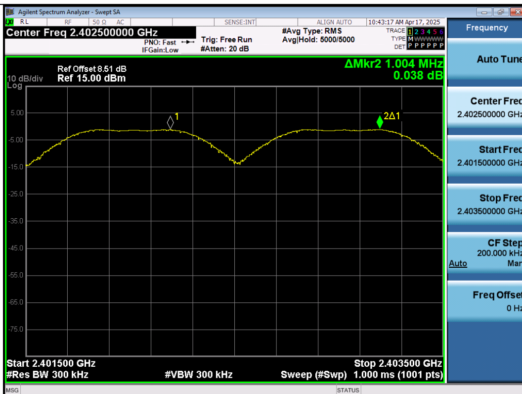
DH5-Ant1-Hop 2402-PASS
