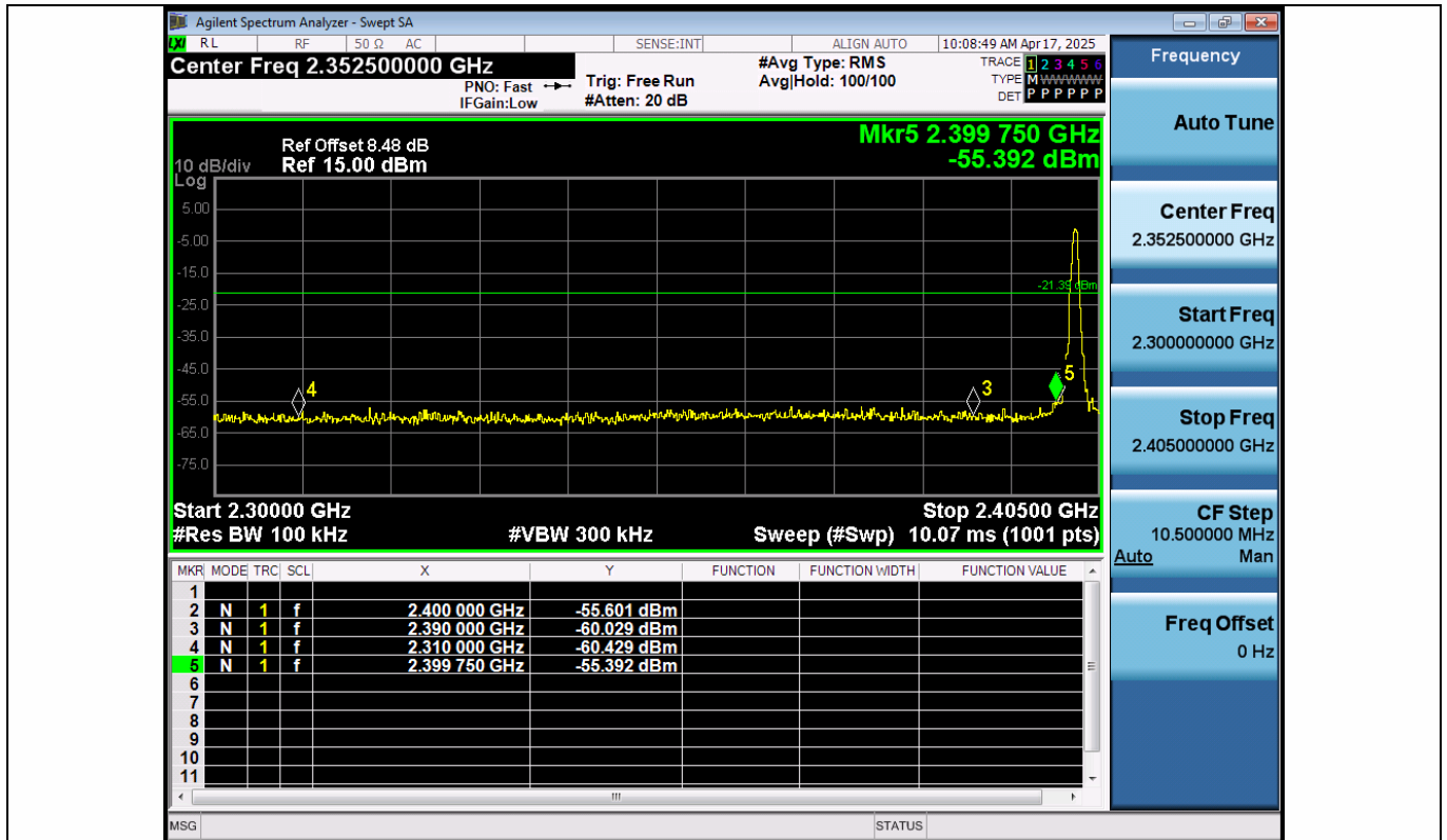
DH5-Ant1-2402-PASS
