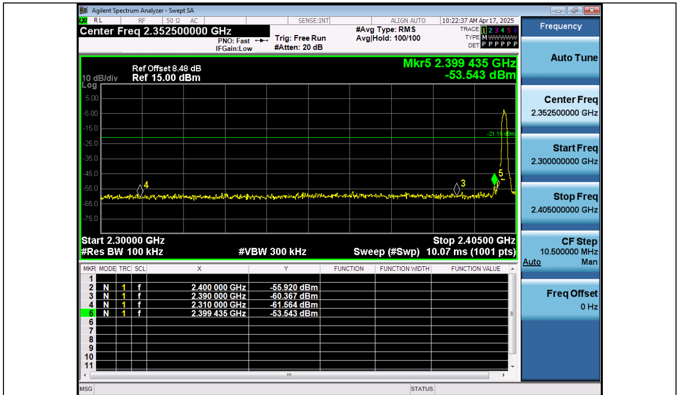
2DH5-Ant1-2402-PASS
