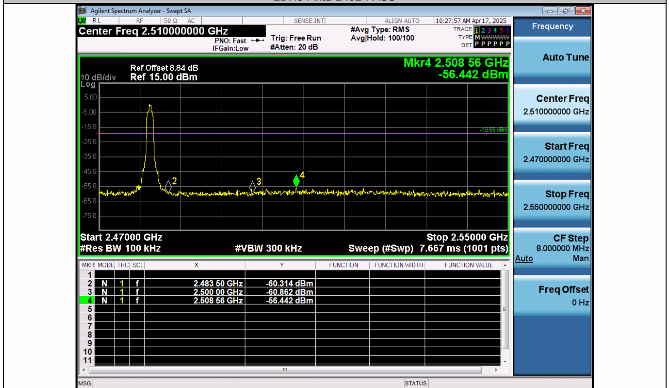
2DH5-Ant1-2480-PASS
