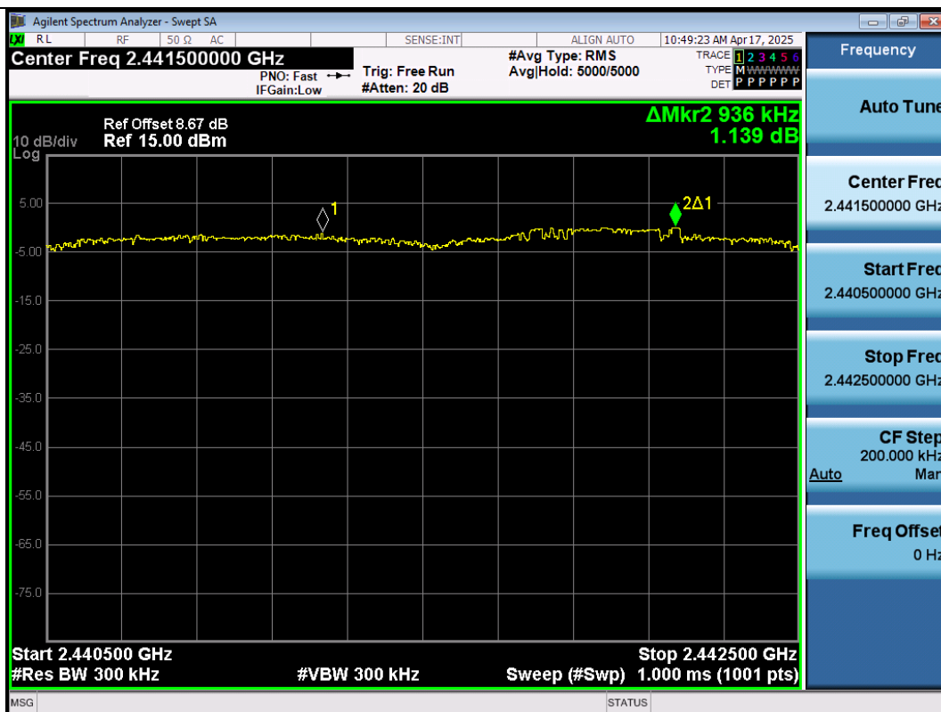
2DH5-Ant1-Hop_2441-PASS
