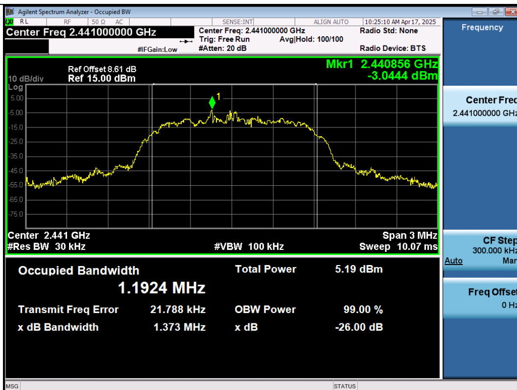
2DH5-Ant1-2441
