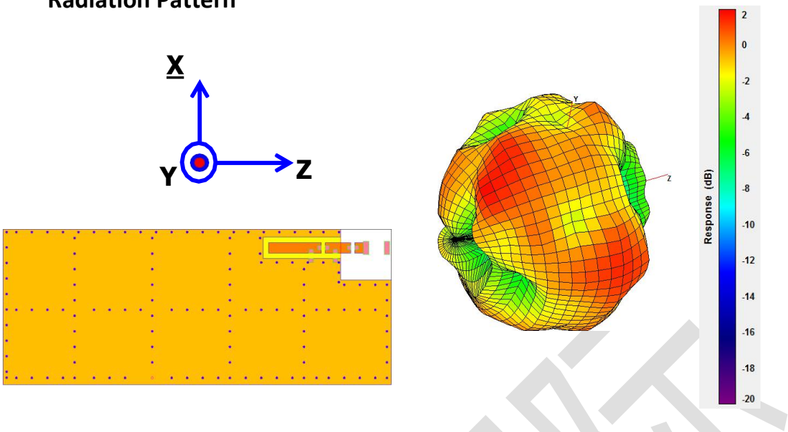
Radiation Pattern
