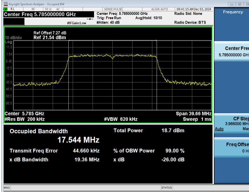
99%_OCB_NVNT_ANT2_802_11n(HT20)_5785
