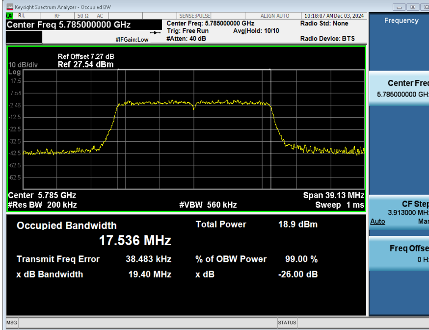
99%_OCB_NVNT_ANT2_802_11ac(VHT20)_5785
