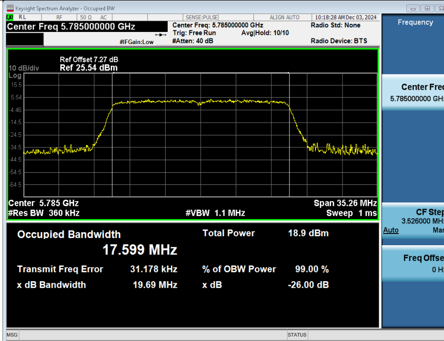
-26BW_NVNT_ANT2_802_11ac(VHT20)_5785
