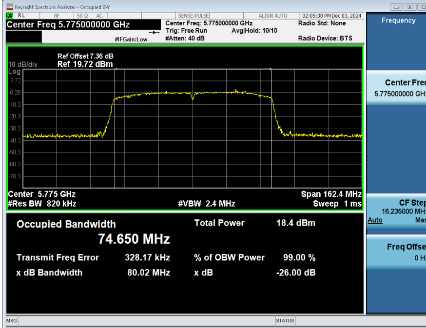
99%_OCB_NVNT_ANT2_802_11ac(VHT80)_5775
