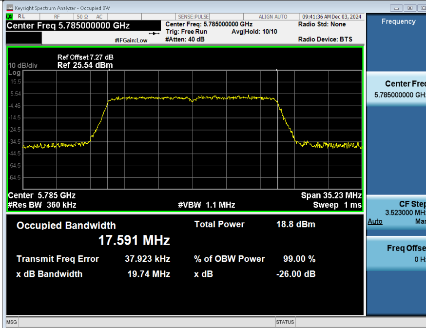
-26BW_NVNT_ANT2_802_11n(HT20)_5785
