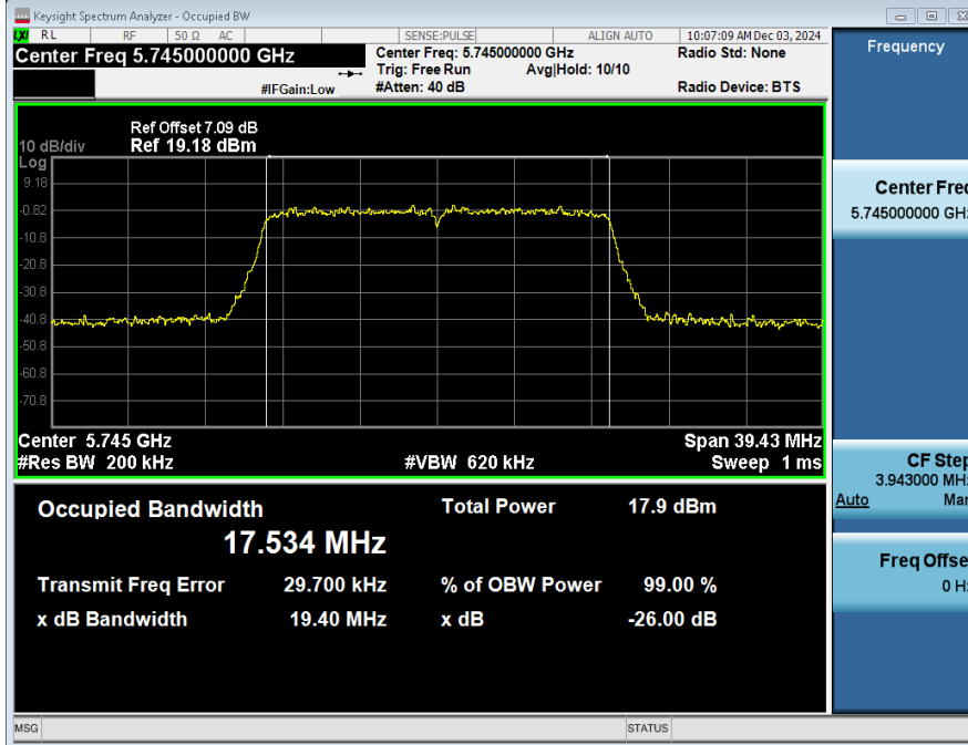
99%_OCB_NVNT_ANT2_802_11ac(VHT20)_5745
