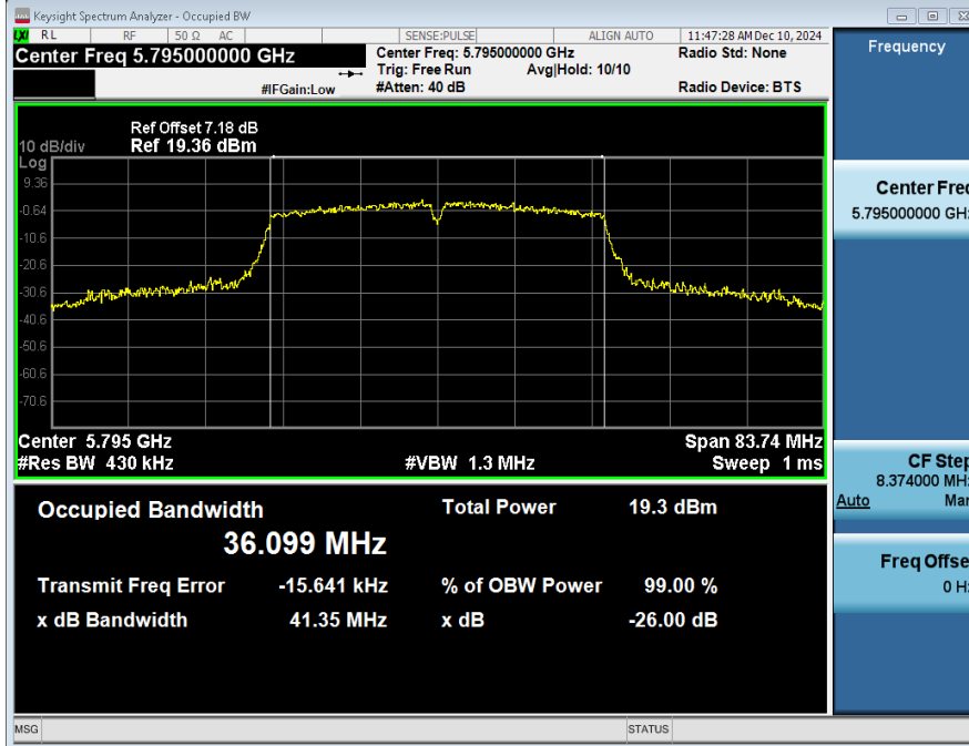
99%_OCB_NVNT_ANT2_802_11n(HT40)_5795
