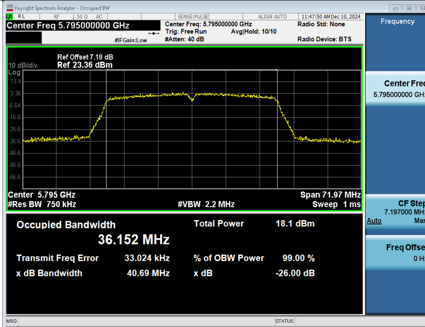
-26BW_NVNT_ANT2_802_11n(HT40)_5795
