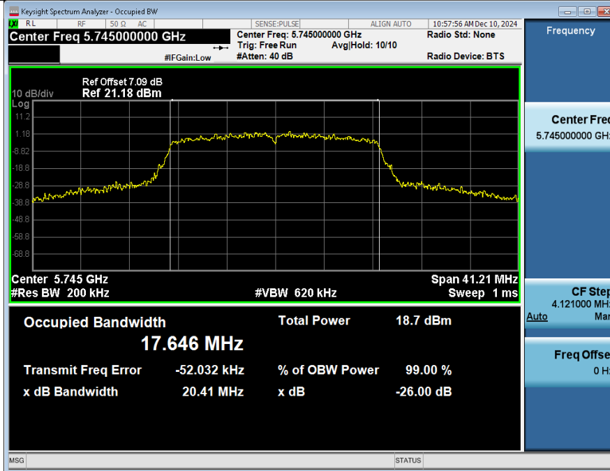
99%_OCB_NVNT_ANT2_802_11ac(VHT20)_5745
