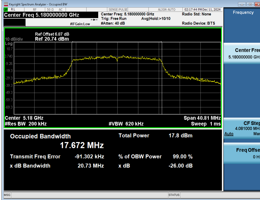
99%_OCB_NVNT_ANT2_802_11n(HT20)_5180
