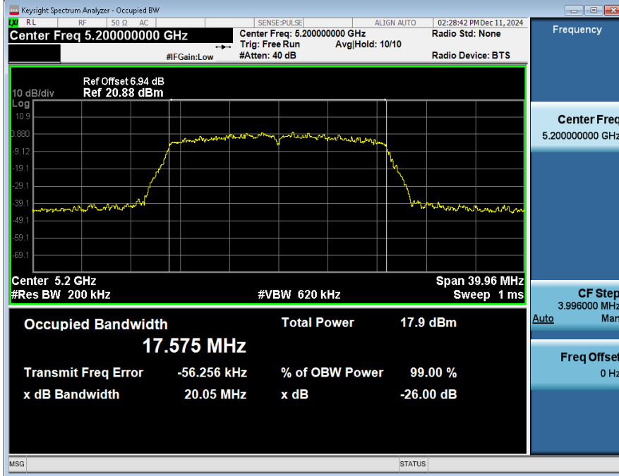
99%_OCB_NVNT_ANT2_802_11n(HT20)_5200
