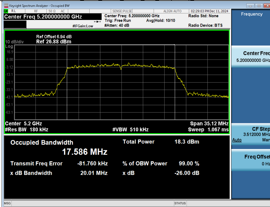
-26BW_NVNT_ANT2_802_11n(HT20)_5200
