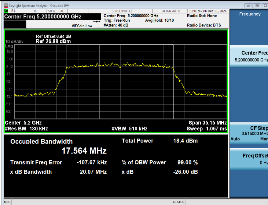
-26BW_NVNT_ANT2_802_11ac(VHT20)_5200
