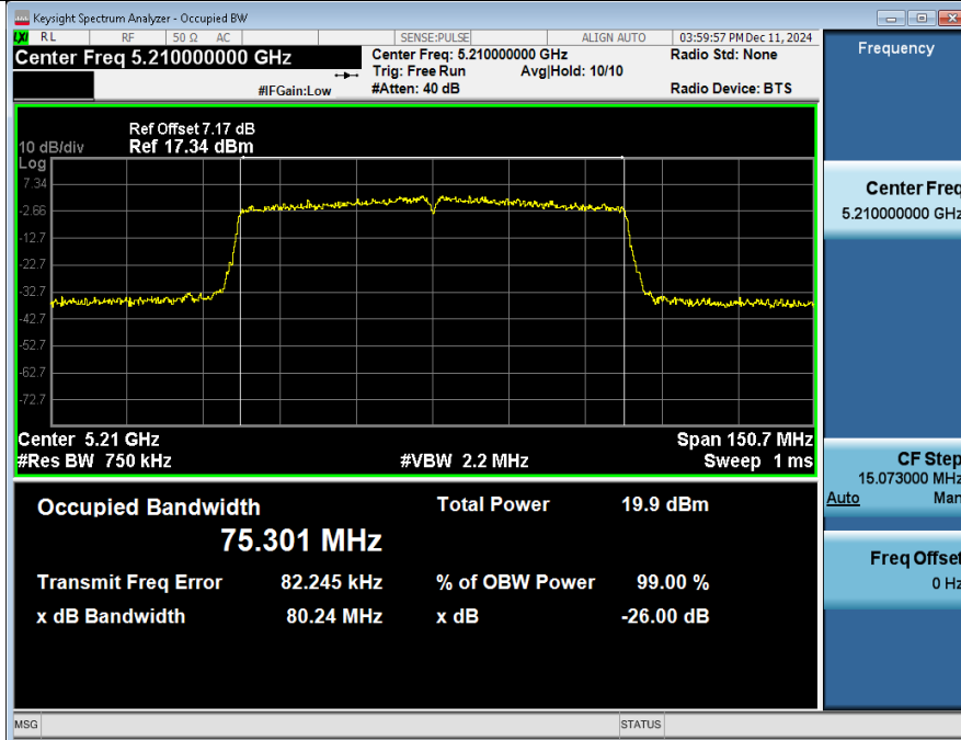
-26BW_NVNT_ANT2_802_11ac(VHT80)_5210
