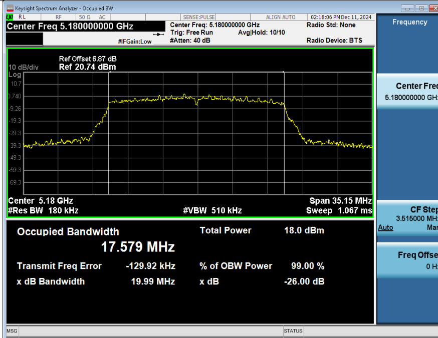
-26BW_NVNT_ANT2_802_11n(HT20)_5180
