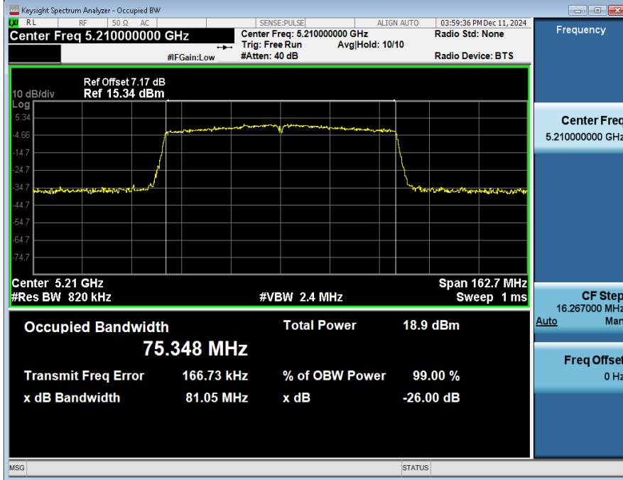
99%_OCB_NVNT_ANT2_802_11ac(VHT80)_5210
