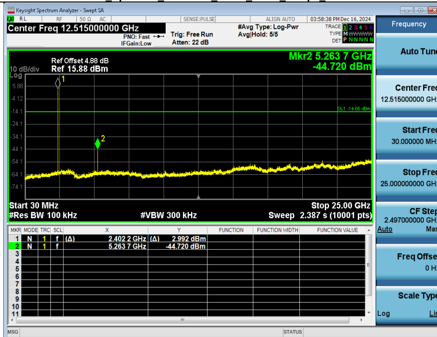
2_Spurious_Emission_NVNT_ANT1_2Mbps_2402
