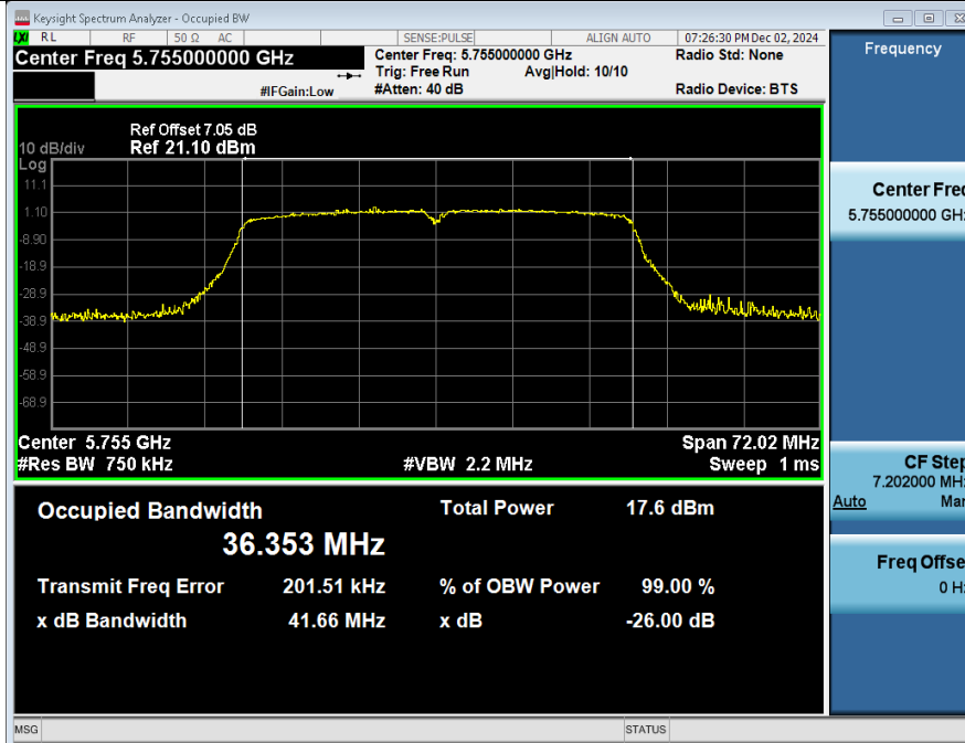
-26BW_NVNT_ANT2_802_11n(HT40)_5755
