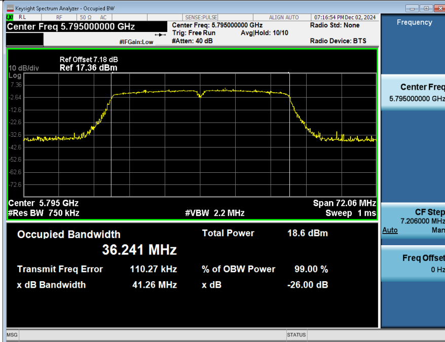
-26BW_NVNT_ANT2_802_11n(HT40)_5795
