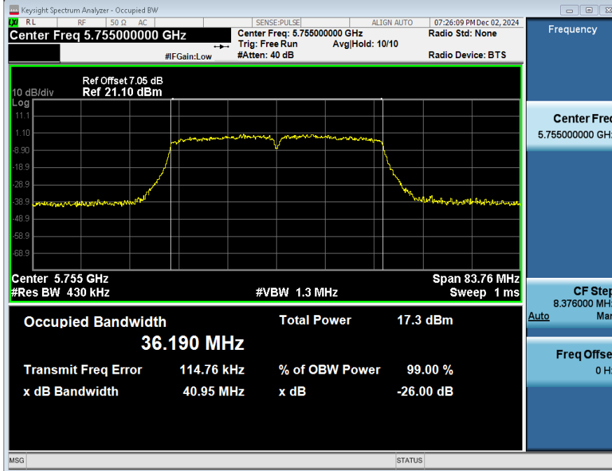
99%_OCB_NVNT_ANT2_802_11n(HT40)_5755
