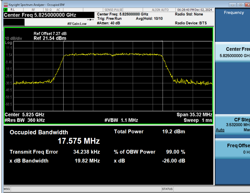
-26BW_NVNT_ANT2_802_11ac(VHT20)_5825
