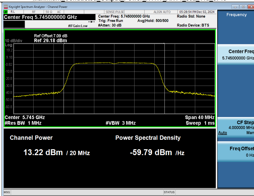
Maximum_Conducted_Output_Power_NVNT_ANT2_802_11a_5745
