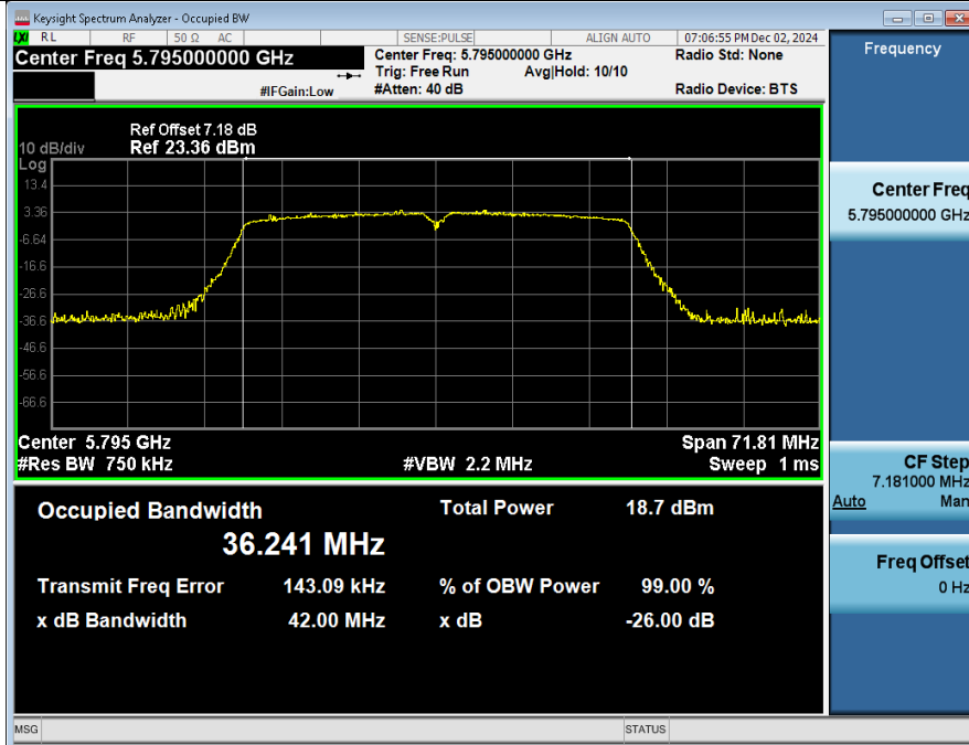
-26BW_NVNT_ANT2_802_11ac(VHT40)_5795
