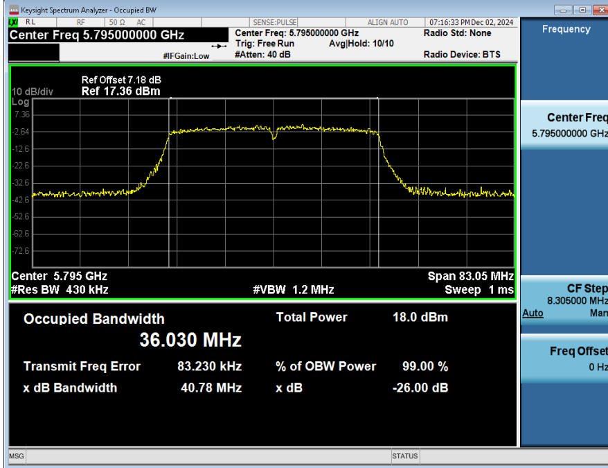
99%_OCB_NVNT_ANT2_802_11n(HT40)_5795
