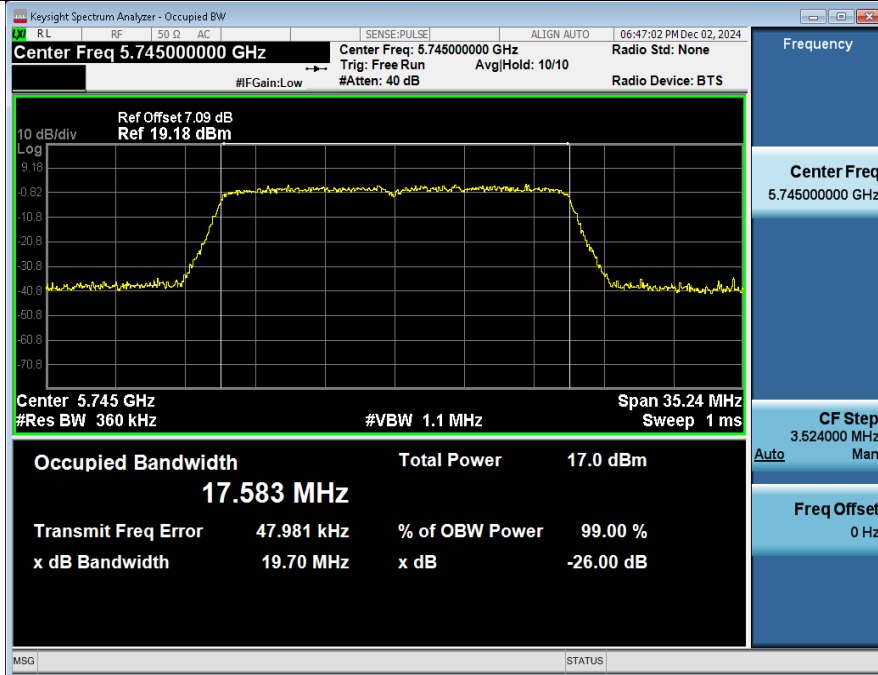
-26BW_NVNT_ANT2_802_11ac(VHT20)_5745
