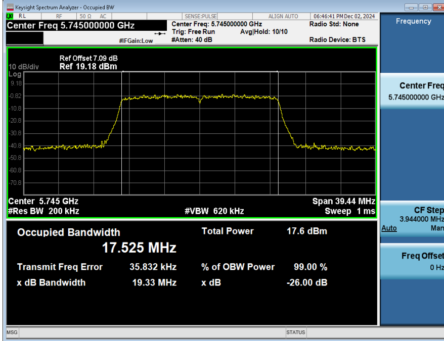
99%_OCB_NVNT_ANT2_802_11ac(VHT20)_5745
