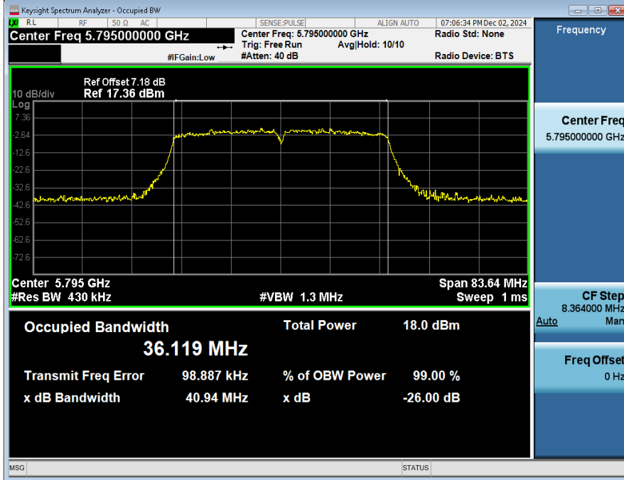
99%_OCB_NVNT_ANT2_802_11ac(VHT40)_5795
