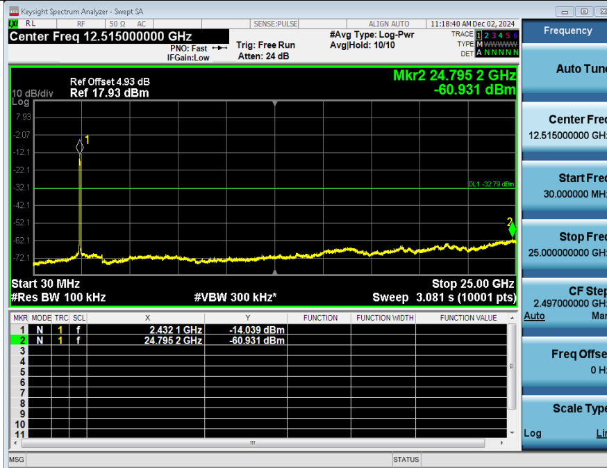
2 Spurious Emission NVNT_ANT2_802_11n(HT40)_2437
