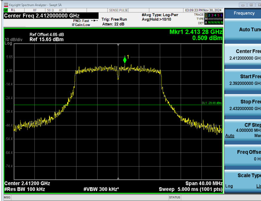
2 Bandedge_NVNT_ANT1_802_11g_2412
