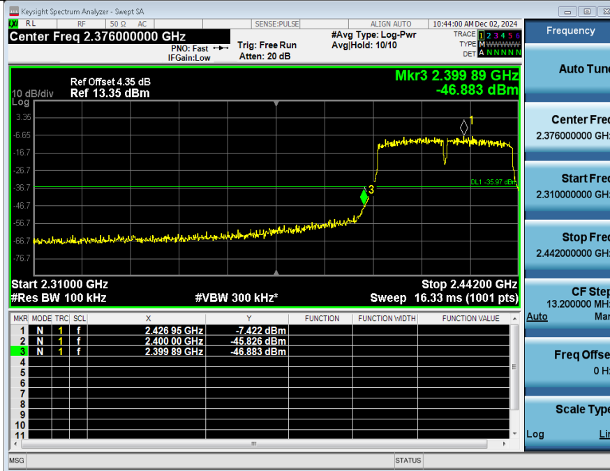
2_Bandedge_NVNT_ANT2_802_11n(HT40)_2422
