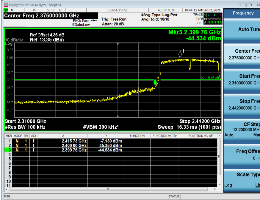
2_Bandedge_NVNT_ANT2_802_11n(HT40)_2422
