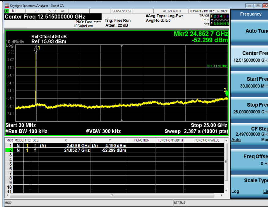
2_Spurious_Emission_NVNT_ANT1_2Mbps_2440
