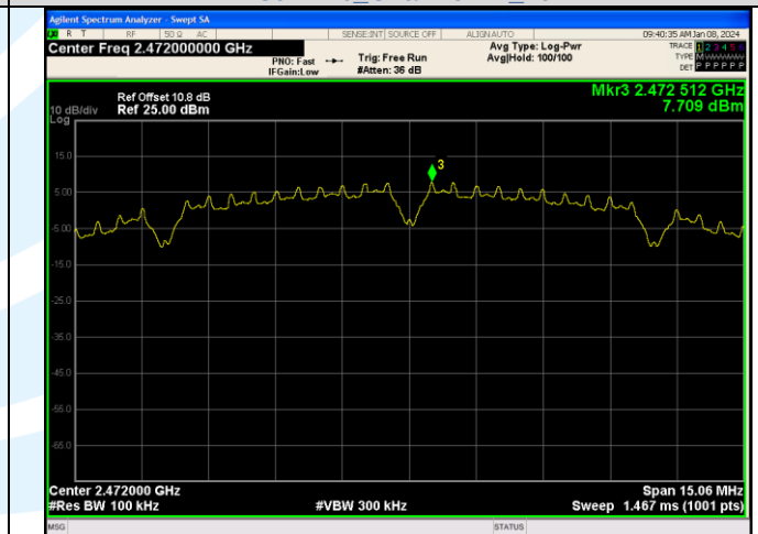
In-Band Reference Level IEEE 802.11b Channel 13 20MHz
