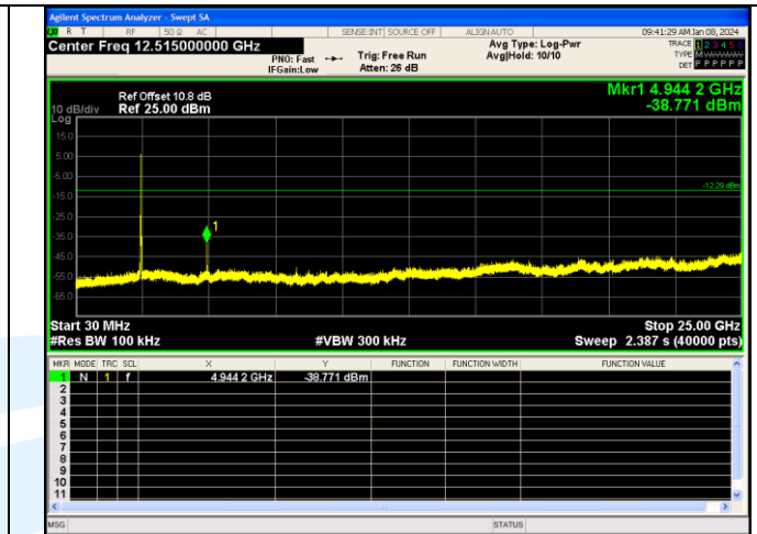
Spurious Emission IEEE 802.11b Channel 13 20MHz
