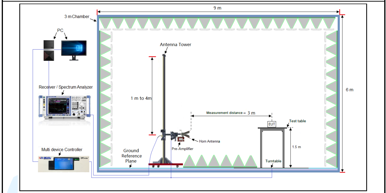
Figure 3. Above 1GHz
