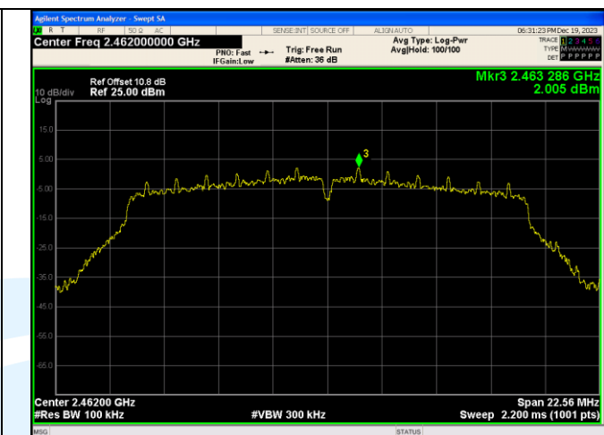
In-Band Reference Level IEEE 802.11g Channel 11 20MHz
