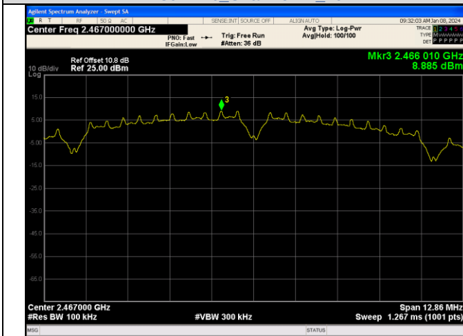
In-Band Reference Level IEEE 802.11b Channel 12 20MHz
