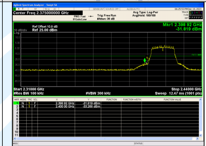
Out Of Band Emission IEEE 802.11g Channel 1 20MHz
