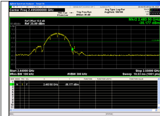
Out Of Band Emission IEEE 802.11b Channel 13 20MHz
