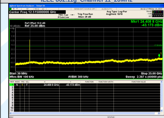
Spurious Emission IEEE 802.11g Channel 11 20MHz
