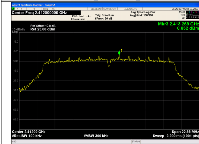
In-Band Reference Level IEEE 802.11g Channel 1 20MHz
