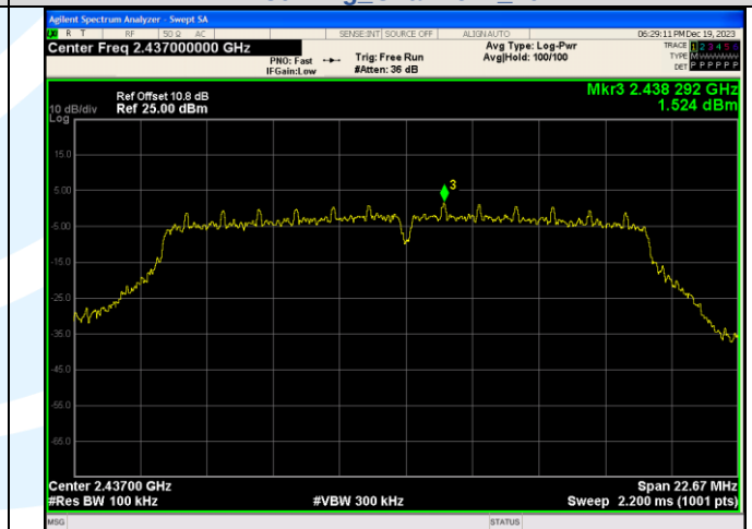
In-Band Reference Level IEEE 802.11g Channel 6 20MHz
