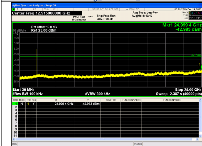
Spurious Emission IEEE 802.11g Channel 1 20MHz
