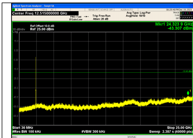
Spurious Emissions IEEE 802.11g Channel 6 20MHz
