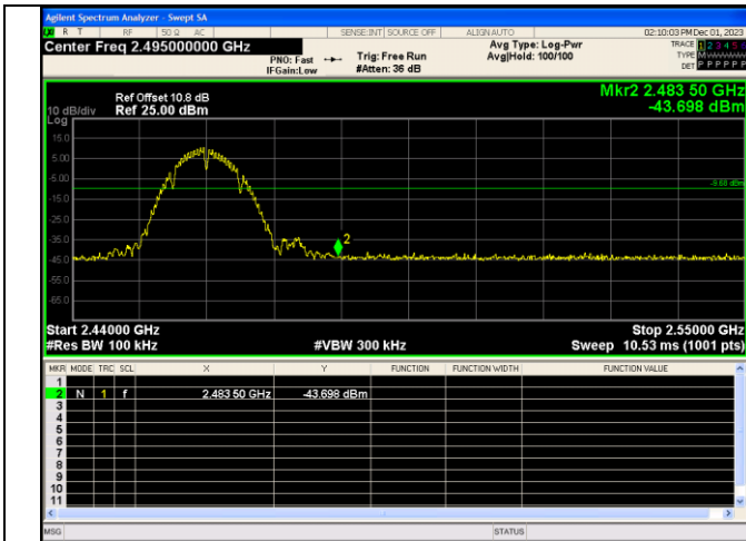
Out Of Band Emission IEEE 802.11b Channel 11 20MHz
