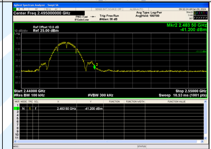
Out Of Band Emission IEEE 802.11b Channel 12 20MHz
