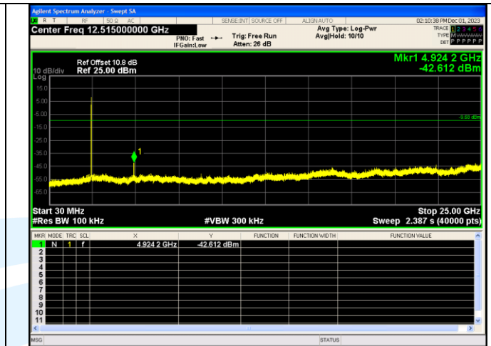
Spurious Emission IEEE 802.11b Channel 11 20MHz
