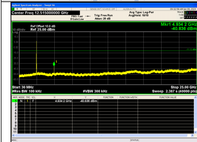
Spurious Emission IEEE 802.11b Channel 12 20MHz
