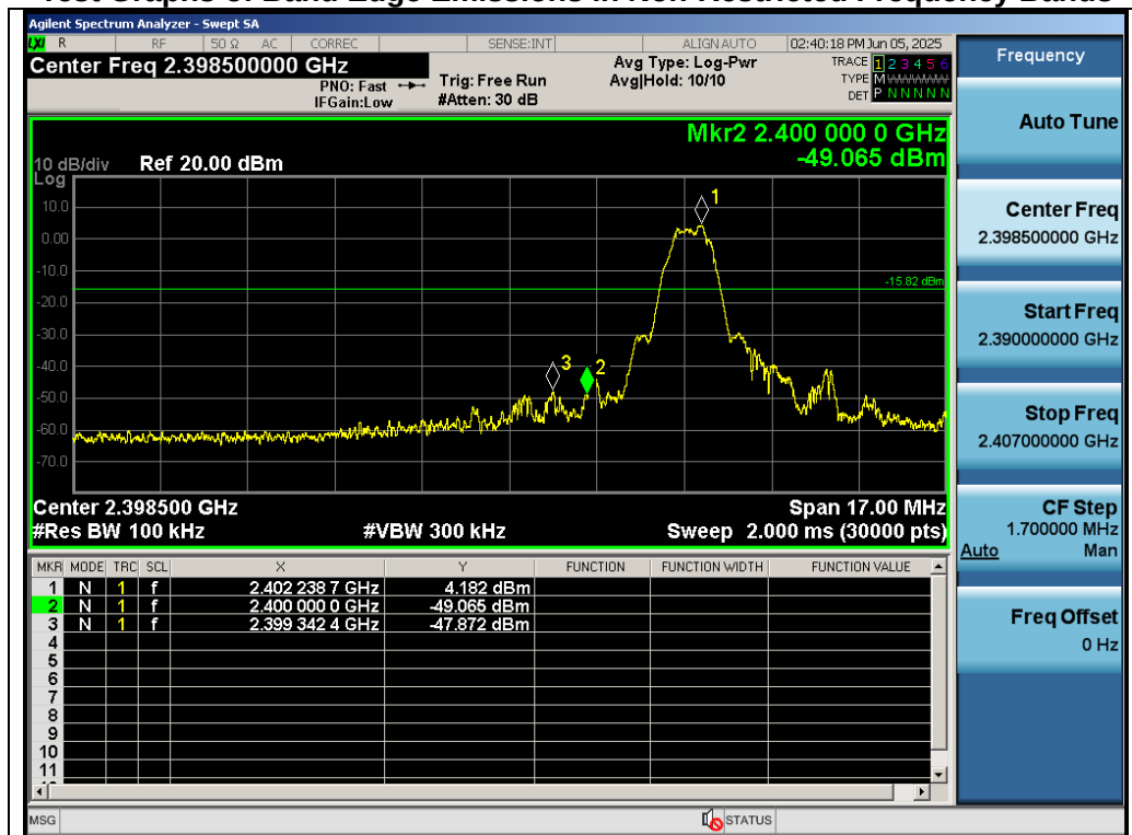
Test_Graph_SRD 2.4G_ANT1_2402_Lower Band Edge Emissions
