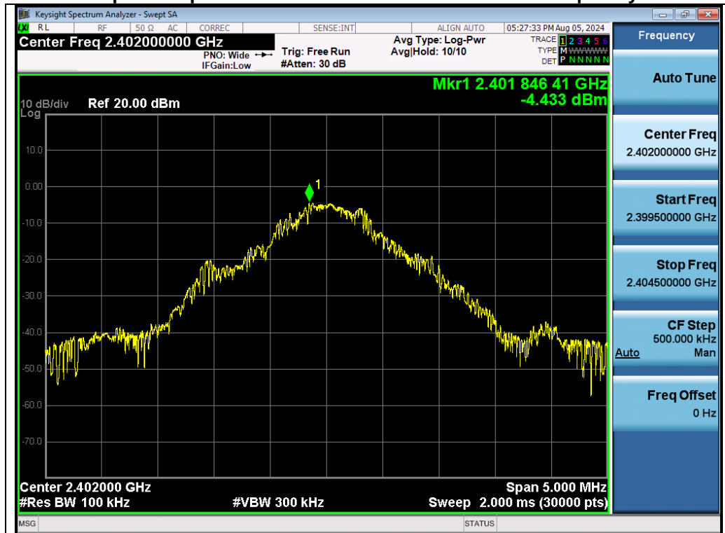
Test_Graph_2.4G_ANT1_2402_GFSK_Reference Level
