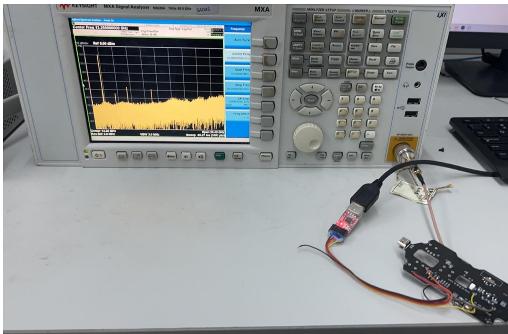
RF CONDUCTED TEST SETUP
