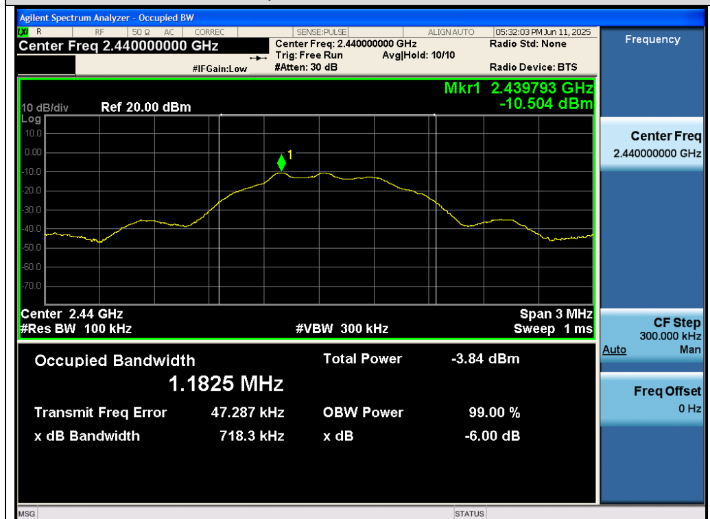
Test_Graph_SRD_ANT1_2440_DTBSW
