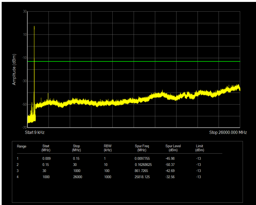
Band5 QAM16 BW=3MHz Channel=20635 RB Size=1 Position=#0 NB Index=0
