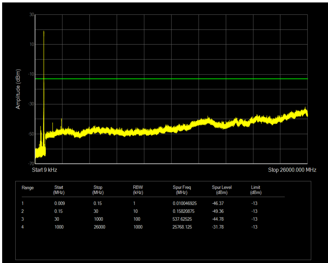
Band5 QPSK BW=10MHz Channel=20450 RB Size=1 Position=#0 NB Index=0
