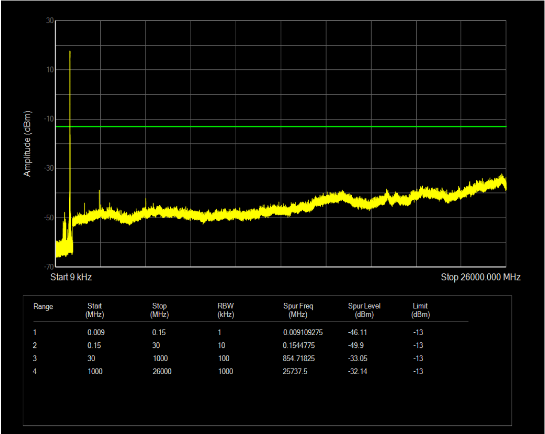
Band5 QAM16 BW=1.4MHz Channel=20643 RB Size=1 Position=#0 NB Index=0
