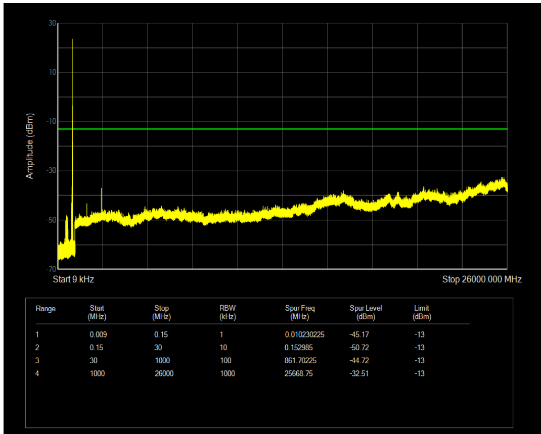
Band5 QAM16 BW=3MHz Channel=20635 RB Size=6 Position=#0 NB Index=0
