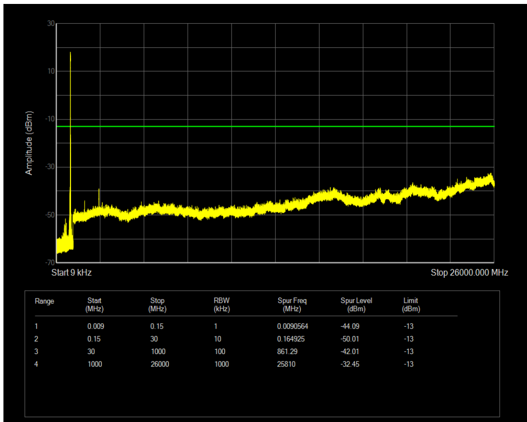
Band5 QPSK BW=5MHz Channel=20425 RB Size=1 Position=#0 NB Index=0
