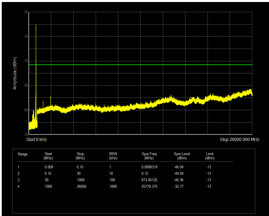
Band5 QAM16 BW=5MHz Channel=20625 RB Size=1 Position=#0 NB Index=0
