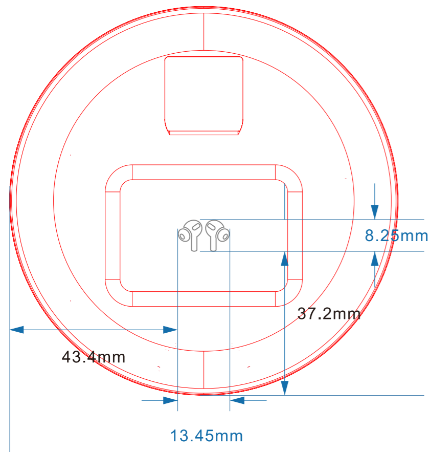
30.15mm Face-piece
