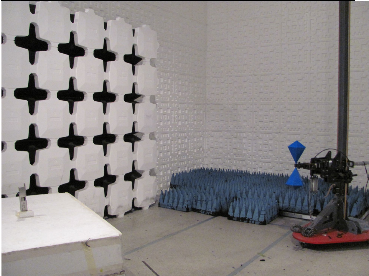
Figure 4. Radiated Emissions Test Setup, 30 MHz to 1000 MHz
