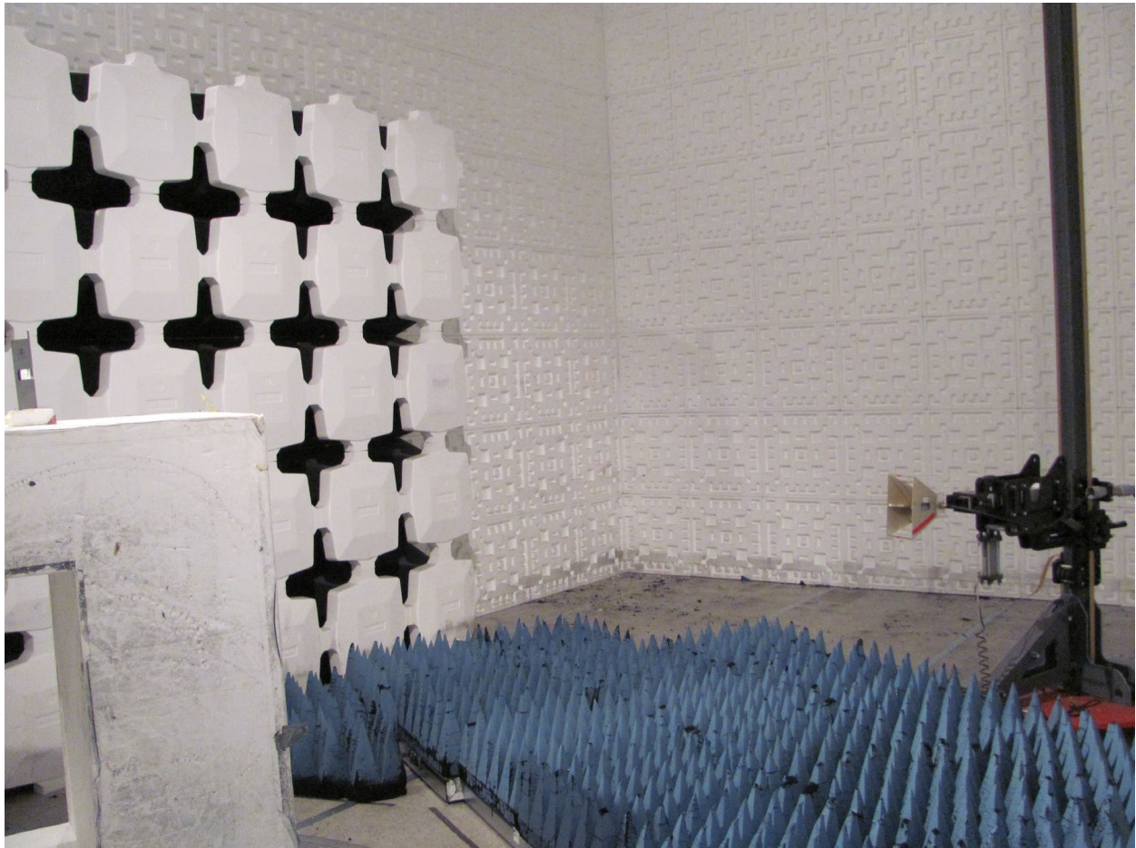
Figure 6. Radiated Emissions Test Setup, 1 GHz to 6 GHz
