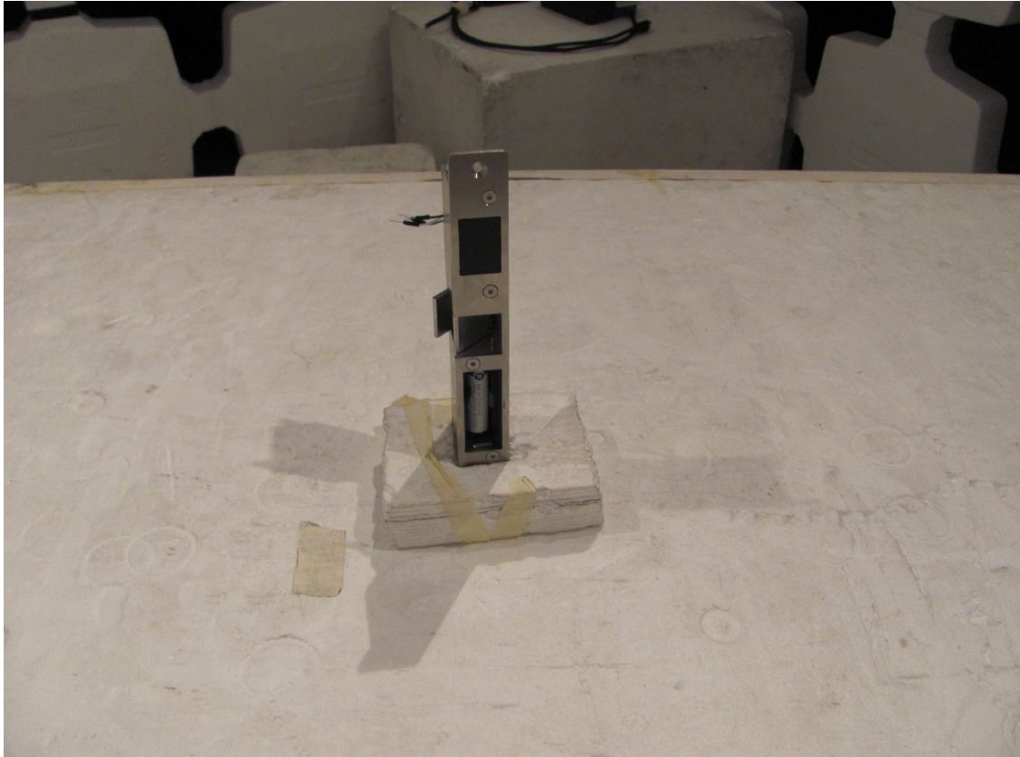
Figure 2. Radiated Emissions Test Setup, Close
