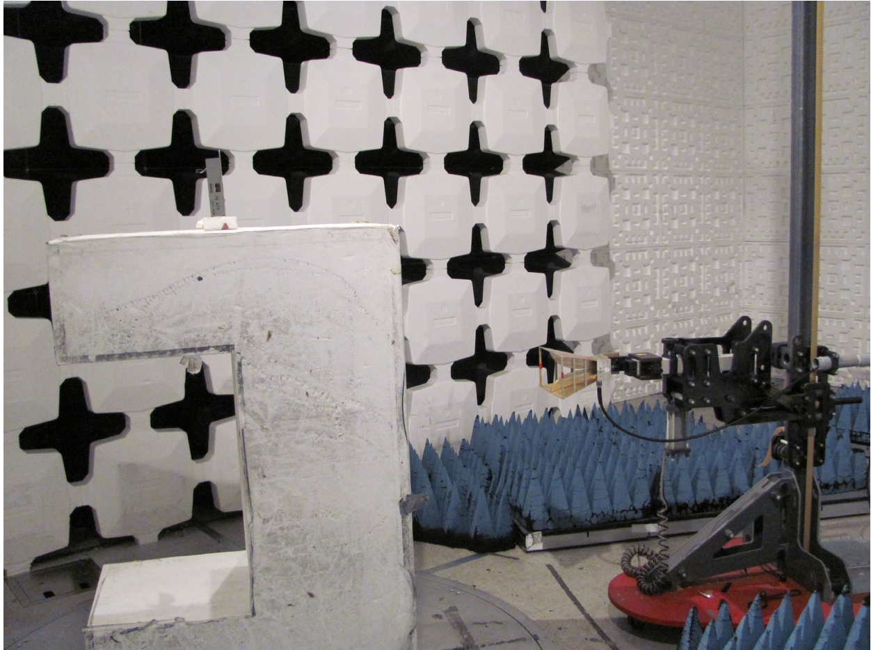
Figure 7. Radiated Emission Test Setup, 6 GHz to 10 GHz
