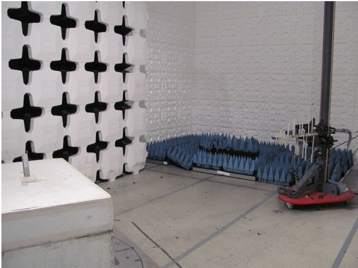
Figure 5. Radiated Emissions Test Setup, Fundamental Emissions
