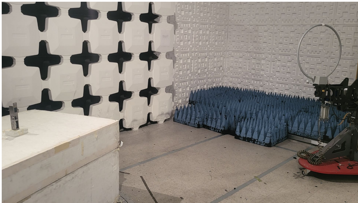
Figure 3. Radiated Emissions Test Setup, 9 kHz to 30 MHz
