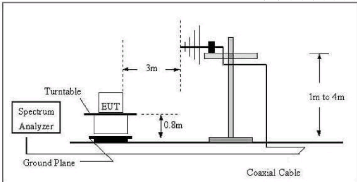
Figure 20. Test Configuration below 1000 MHz
