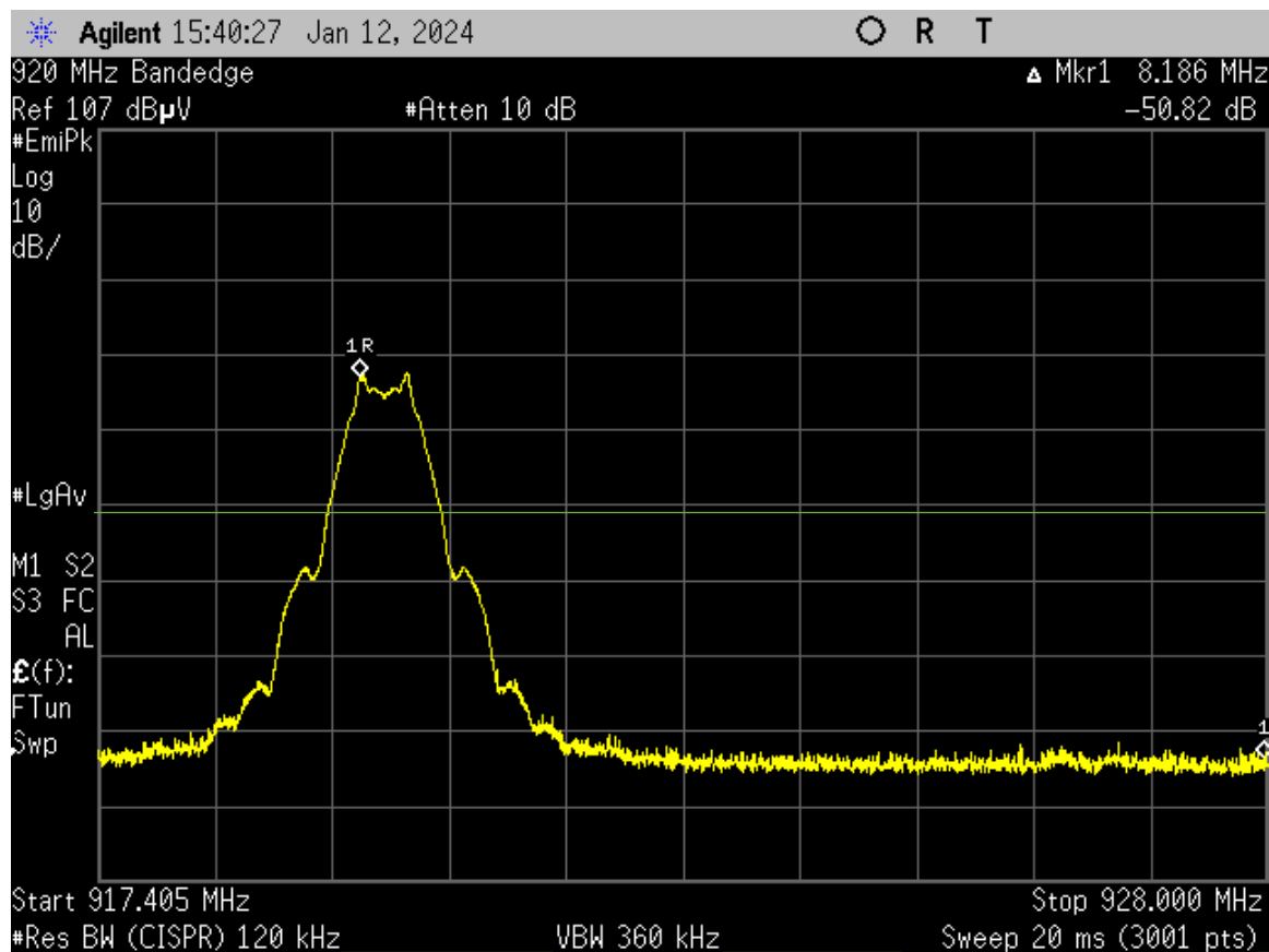
Figure 9. Band Edge Compliance, High Channel Delta – Peak
