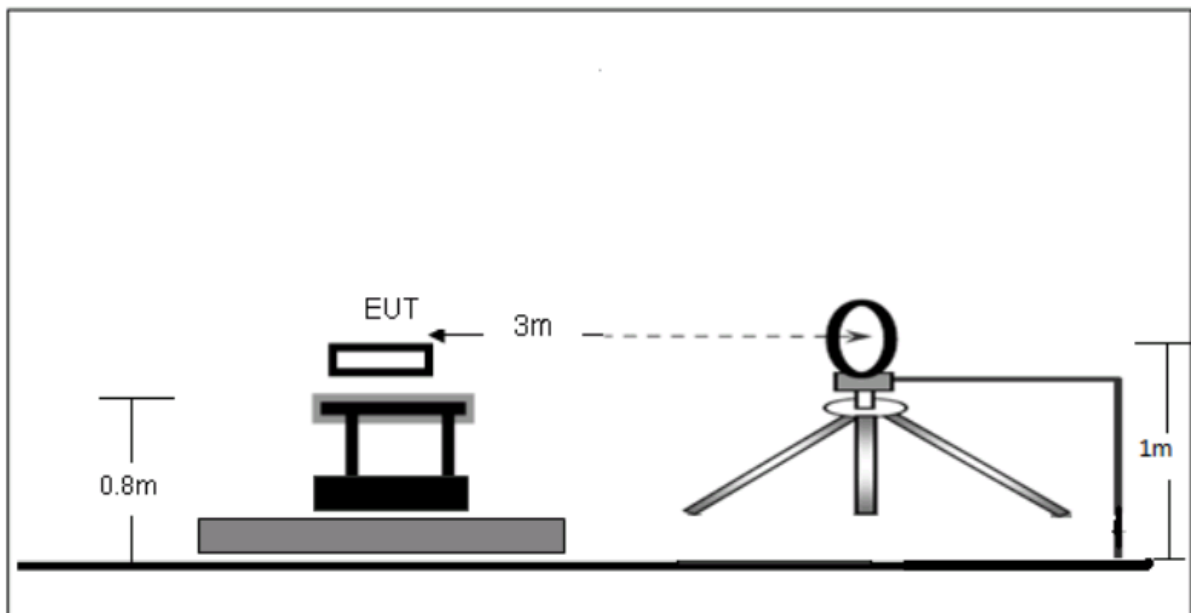
Figure 19. Test Configuration below 30 MHz
