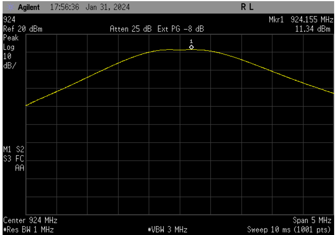
Figure 15. Peak Antenna Conducted Output Power, High Channel
