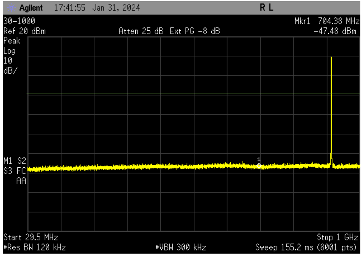
Figure 3. Conducted Spurious Emissions-Mid Channel, 30MHz – 1 GHz
