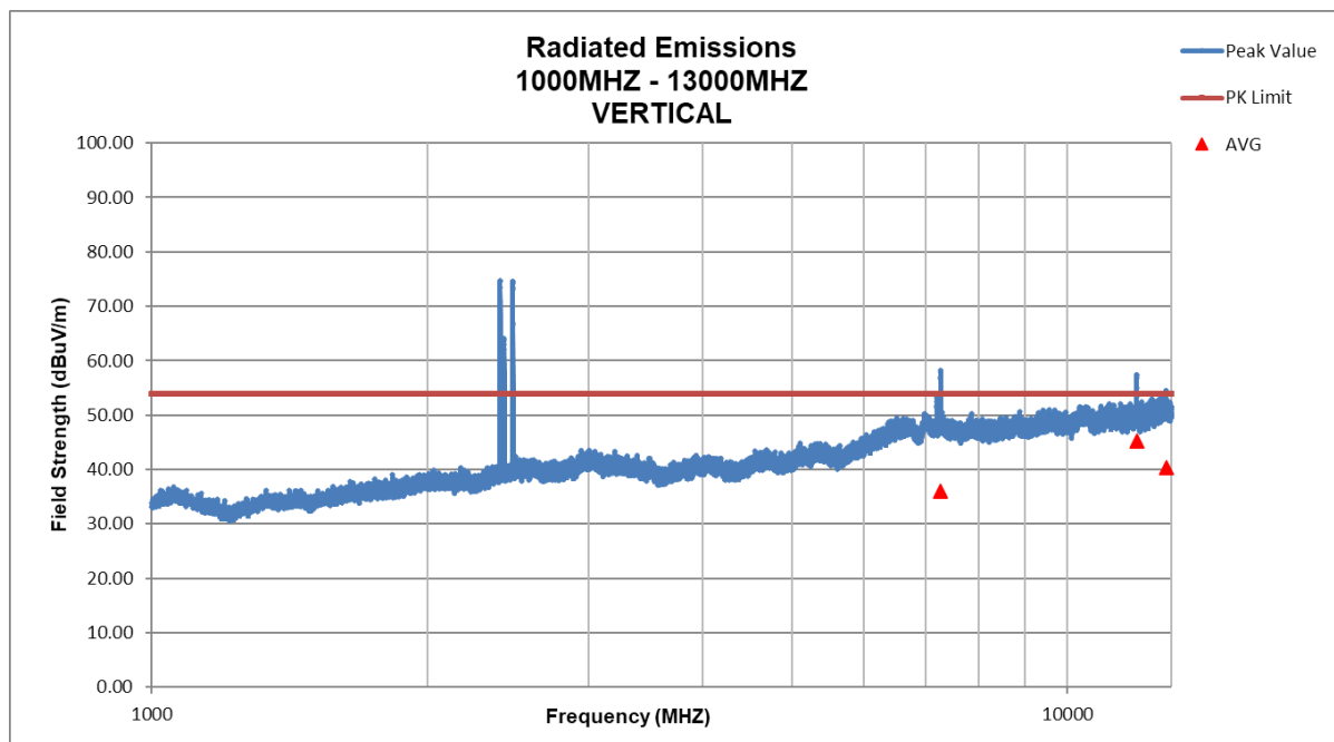
Figure 25. Radiated Emissions TX, 1000 MHz - 13000 MHz - Vertical
