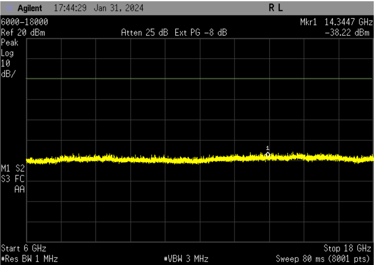
Figure 5. Conducted Spurious Emissions - Mid Channel, 6 GHz – 18 GHz
