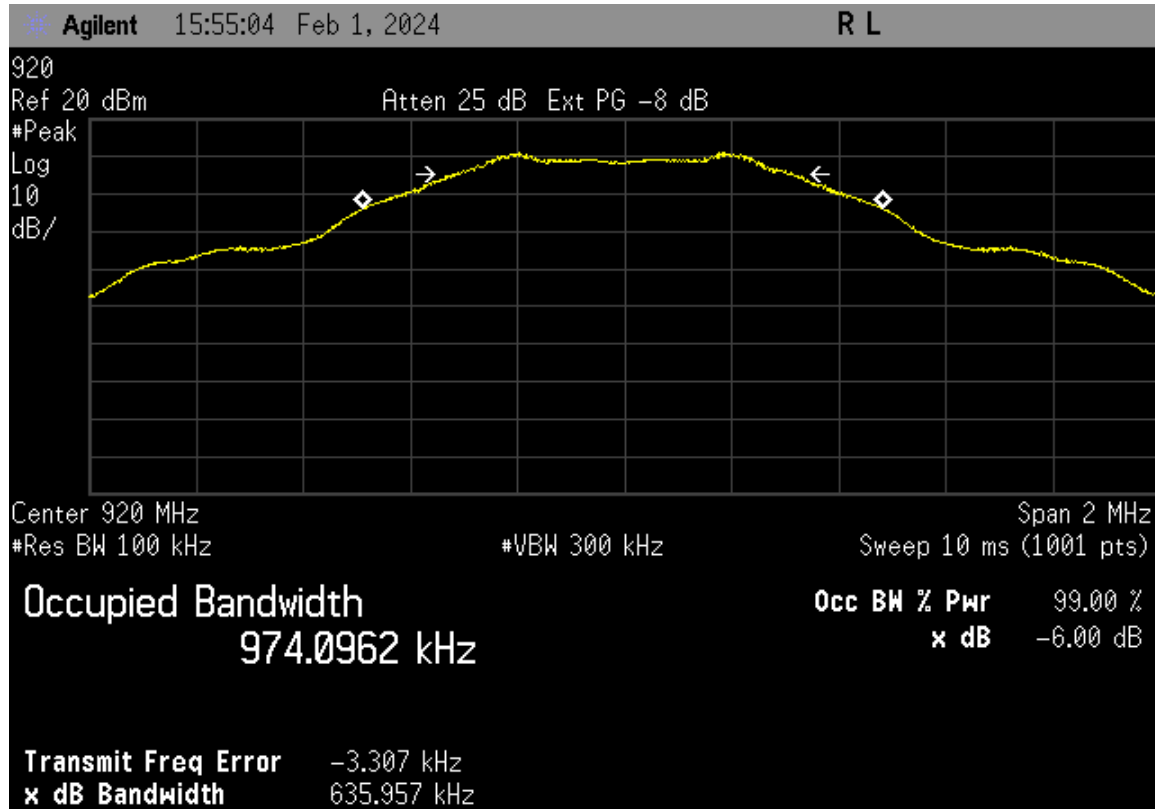
Figure 12. Bandwidth – High Channel
