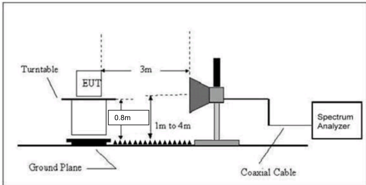
Figure 7. Radiated Emissions Setup (Radiated Bandedge & Restricted Band)
