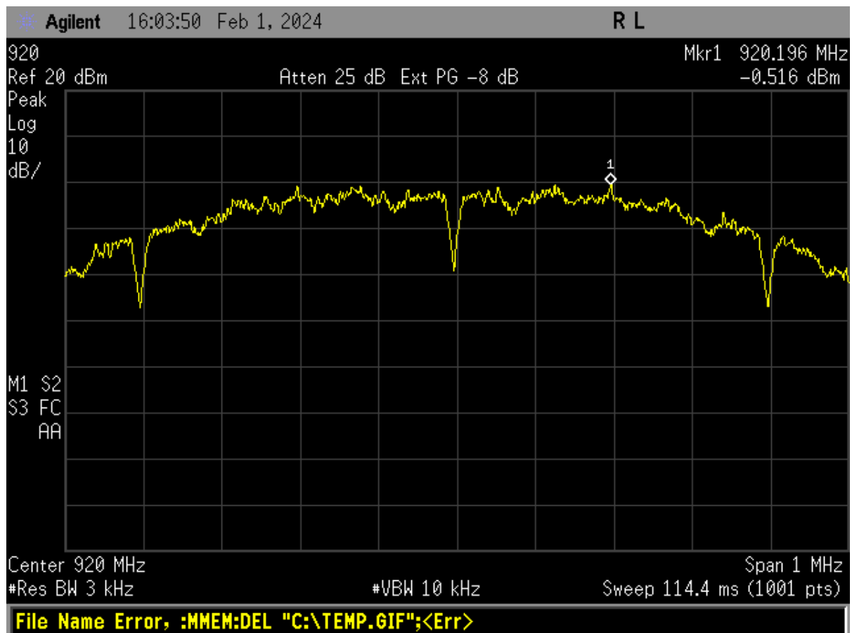
Figure 18. Power Spectral Density, High Channel
