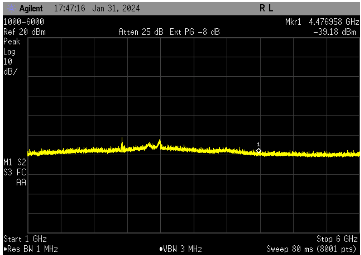
Figure 4. Conducted Spurious Emissions - Mid Channel, 1 GHz – 6 GHz
