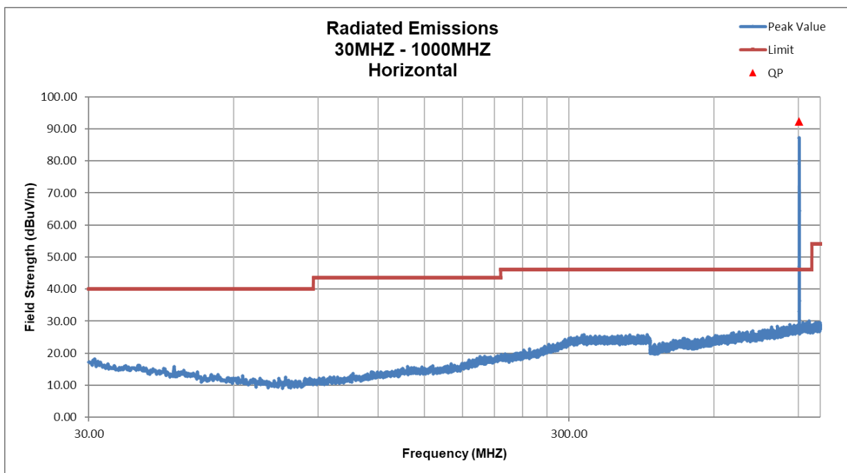
Figure 22. Radiated Emissions TX, 30 MHz - 1000 MHz - Horizontal
