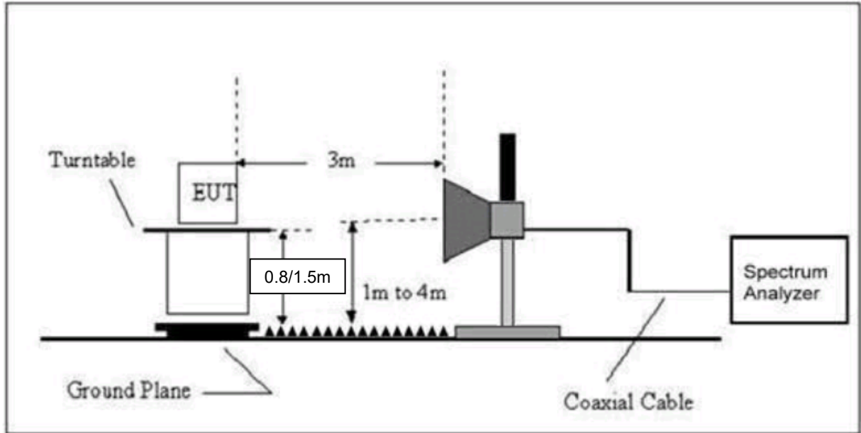
Figure 6. Radiated Emissions Setup (Fundamental and Harmonics)
