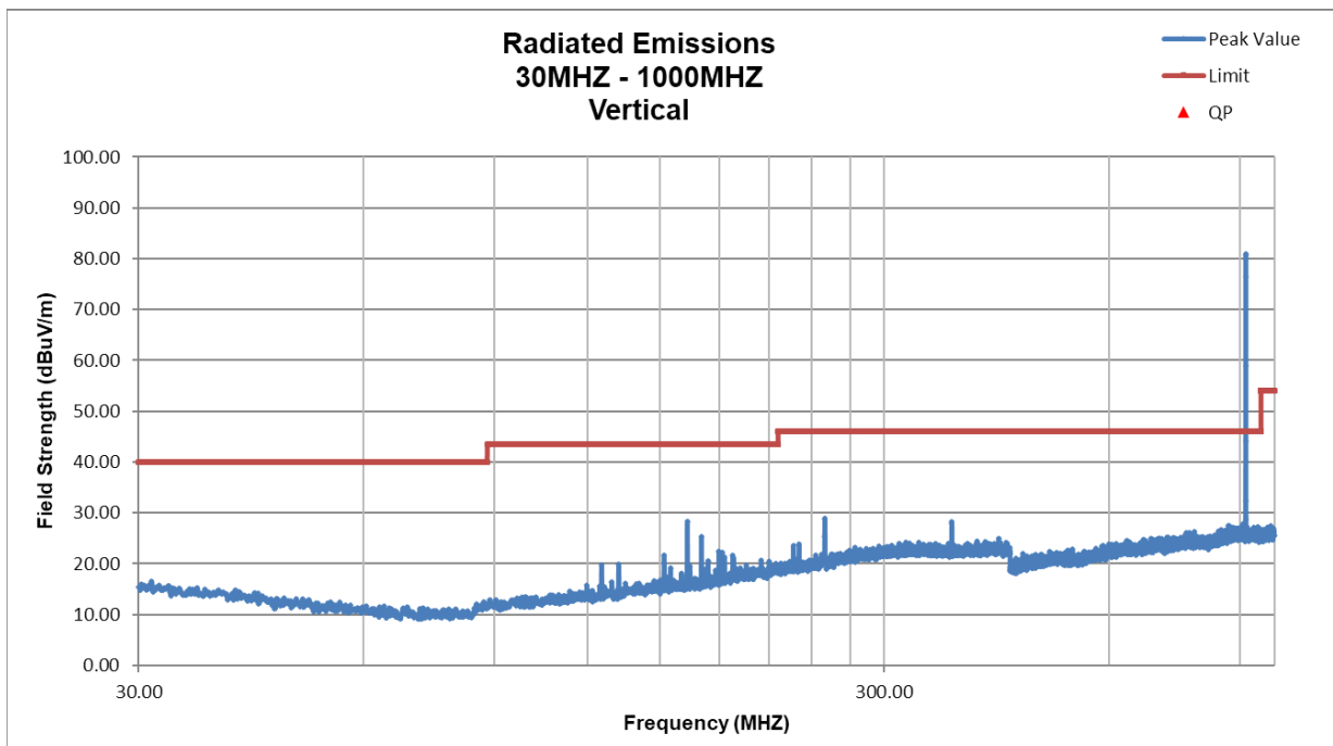
Figure 23. Radiated Emissions TX, 30 MHz - 1000 MHz - Vertical
