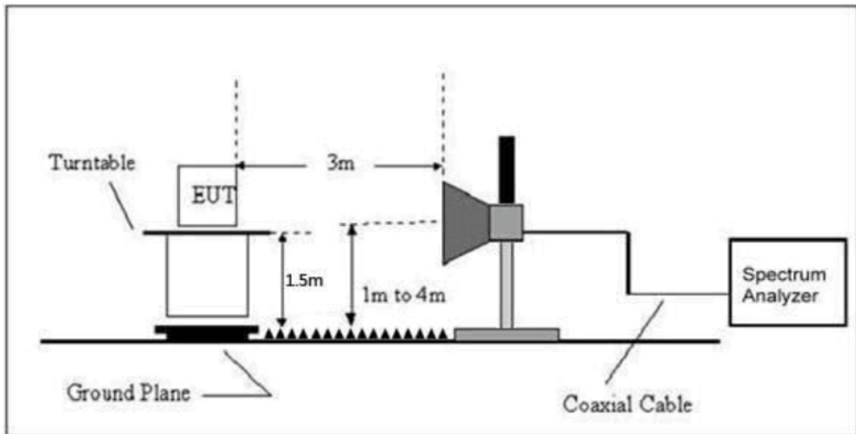
Figure 21. Test Configuration above 1000 MHz
