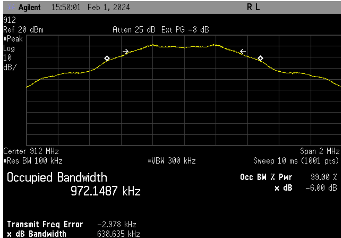
Figure 11. Bandwidth – Low Channel
