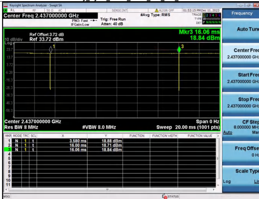
Duty_Cycle_NVNT_ANT1_802_11b_2437
