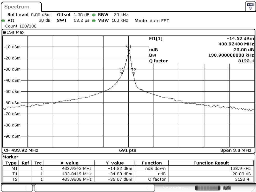
20dB Bandwidth
