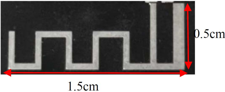
Antenna Photo & Length (cm)
