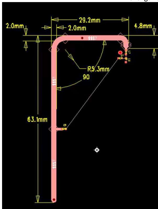
The length of wire antenna
