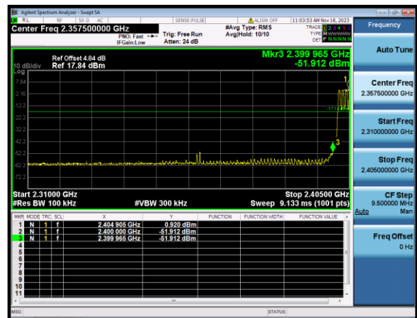
GFSK Hopping
