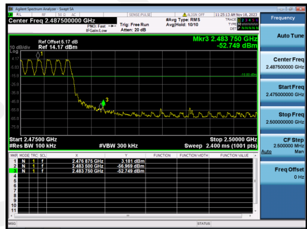
GFSK Hopping
