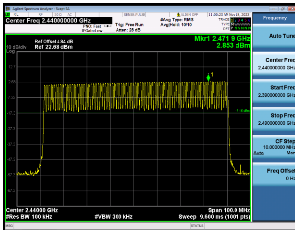
GFSK Hopping
