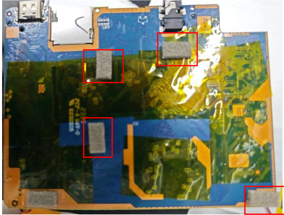
主板漏铜区域贴导电海绵接地 The copper leakage area of the mainboard is grounded with conductive sponge
