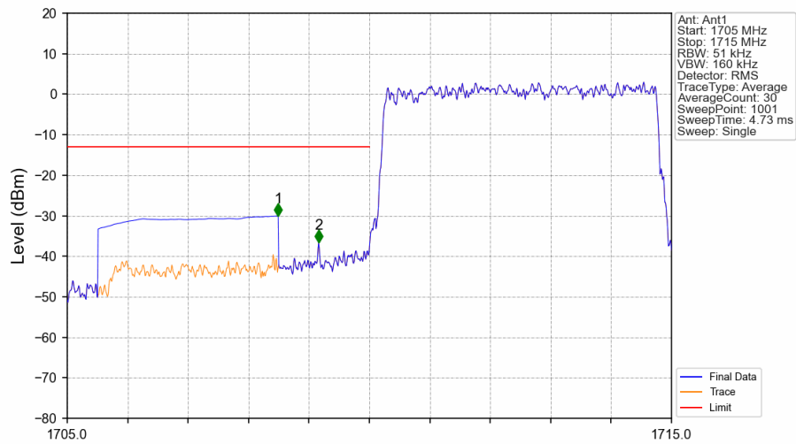
Band66_5MHz_QPSK_LCH_1712.5MHz_RB_25_0_NTNV
