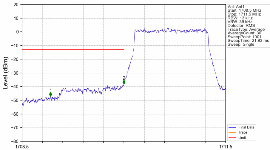
Band66_1.4MHz_QPSK_LCH_1710.7MHz_RB_6_0_NTNV
