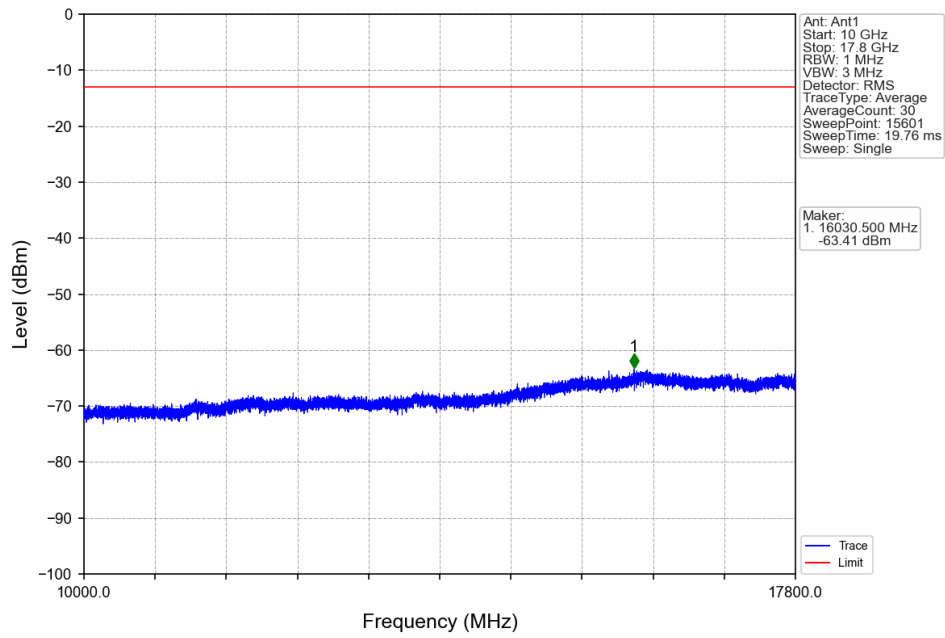
Band66_1.4MHz_QPSK_LCH_1710.7MHz_RB_6_0_NTNV
