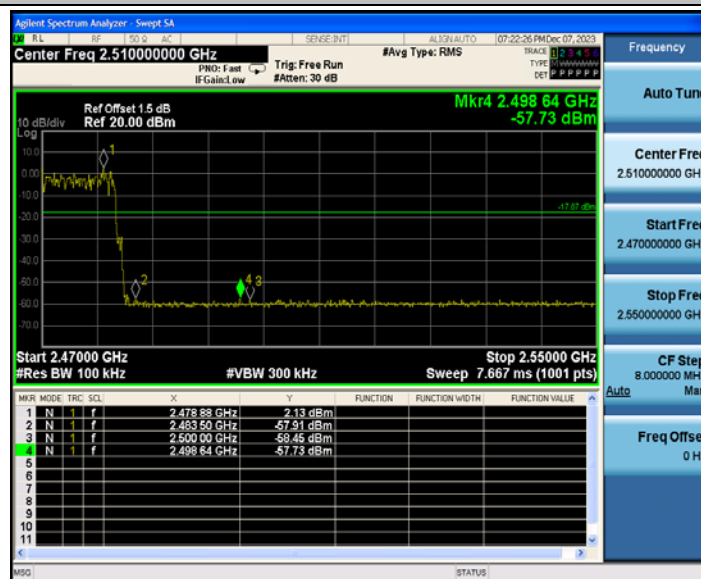
8-DPSK_High_Hop_2480
