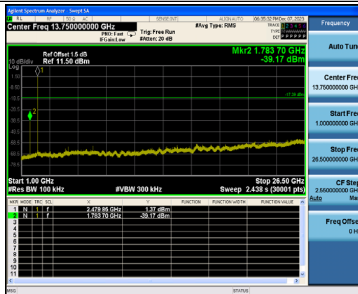
8-DPSK_2402_0-Reference
