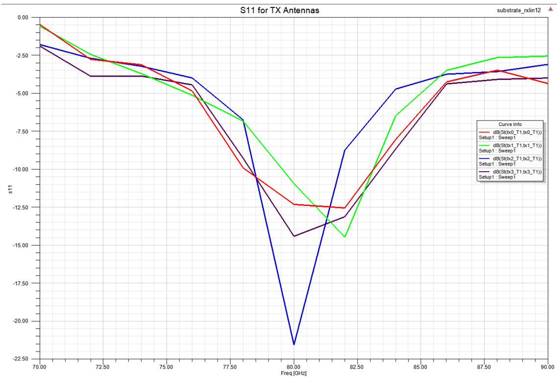
Figure 2 S11 for TX Antennas
