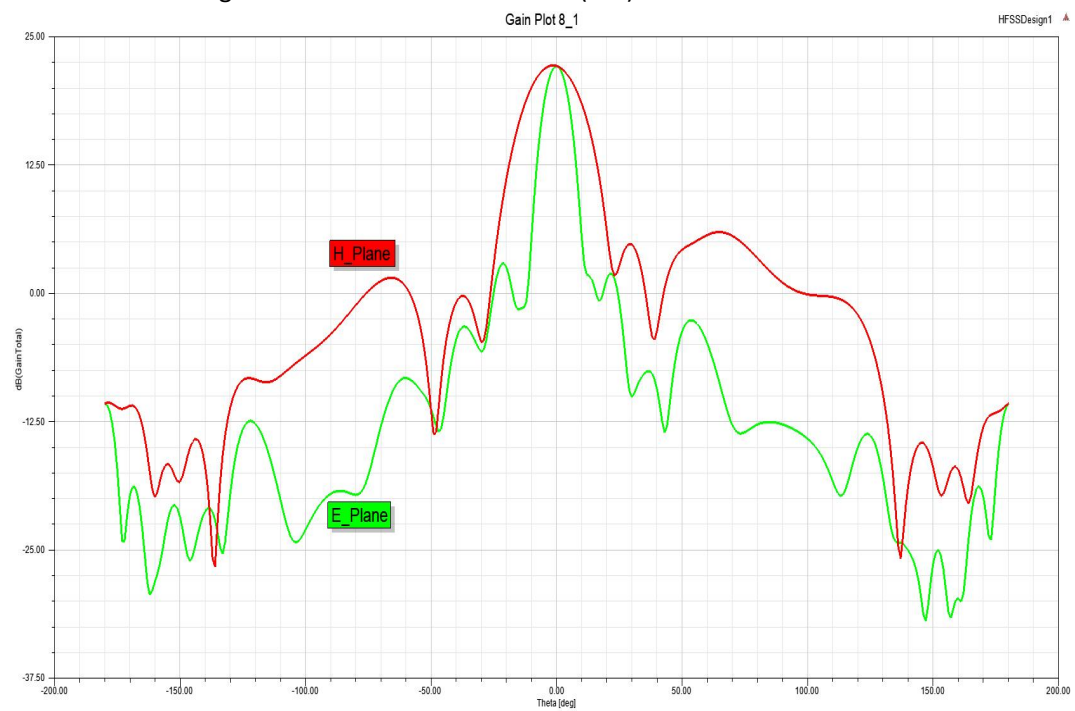
Figure 8 Radiation Pattern for Tx2(Tx3) Antennas at 77.5GHz
