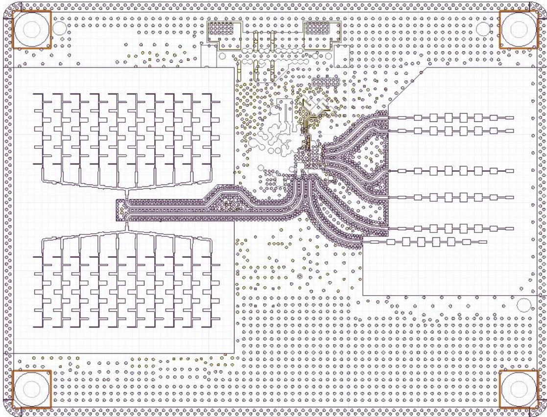
Figure 1 relative position of antenna on the top layer of board
