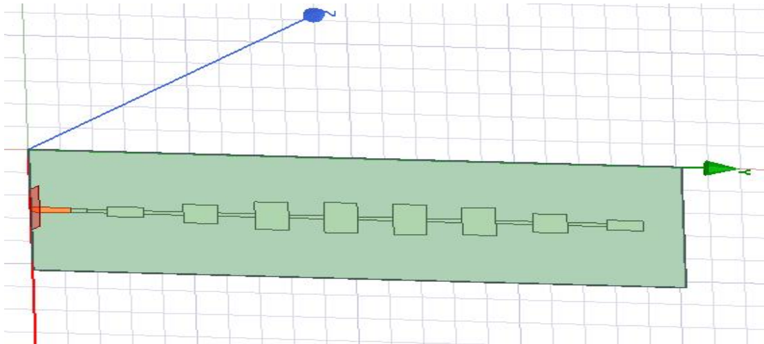
Figure 4 Tx Antenna(Tx0 Tx1)
