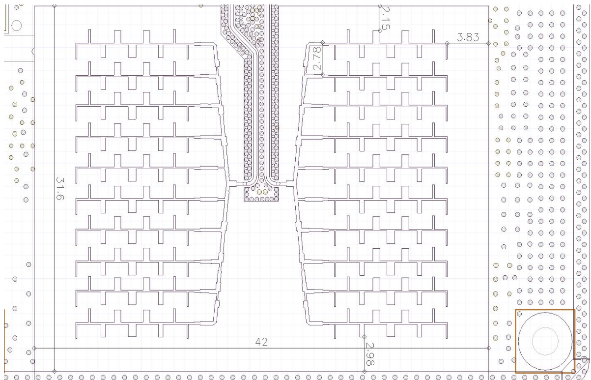
Figure 3 dimension (Tx2 Tx3)
