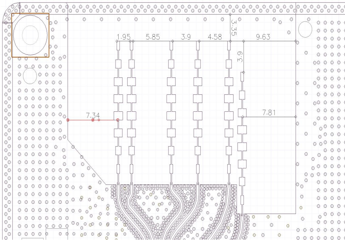
Figure 2 dimension (Rx0 Rx1 Rx2 Rx3 Tx0 Tx1)
