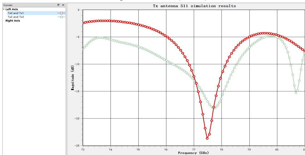
Figure 6 Tx Antenna S11
