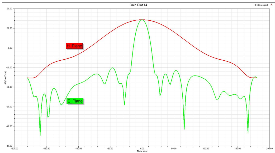
Figure 7 Radiation Pattern for Tx0(Tx1) Antennas at 77.5GHz
