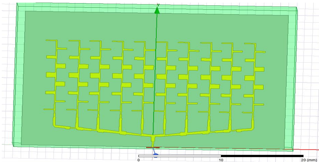
Figure 5 Tx Antenna(Tx2 Tx3)
