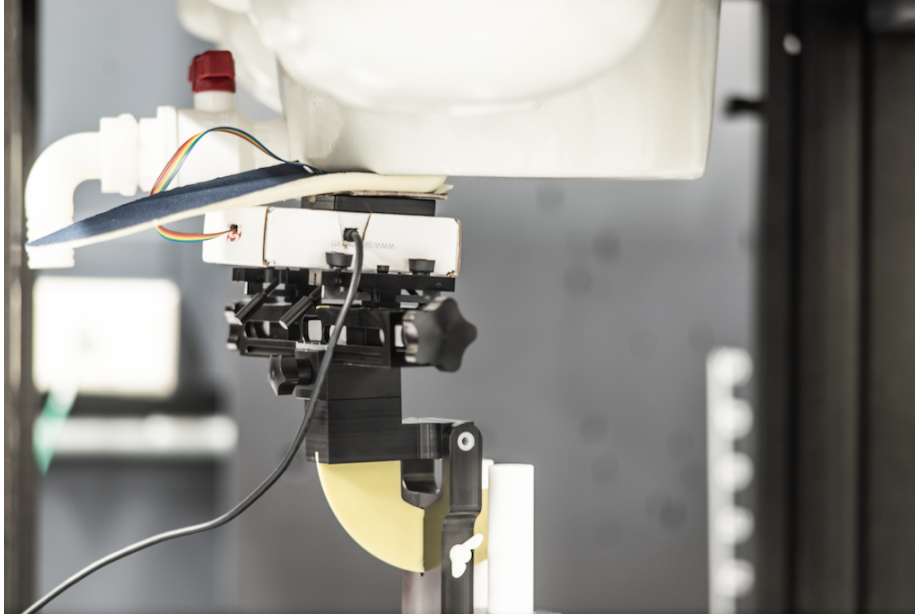
Figure A SAR Test Setup (Side View)
