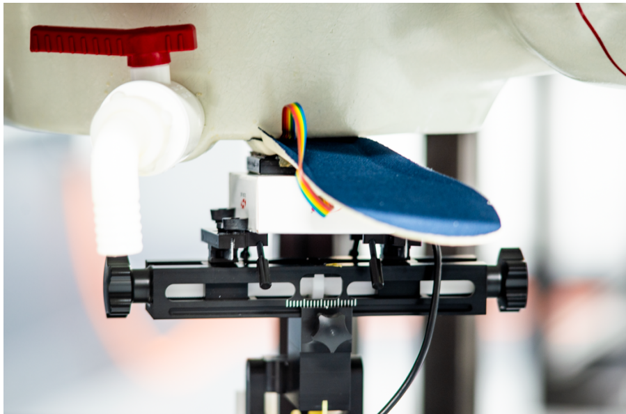
Figure B SAR Test Setup (Front View)
