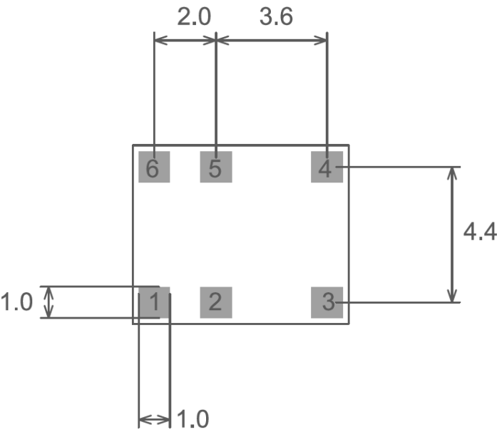
Pads 1-6 = 1.0 x 1.0 (mm)
