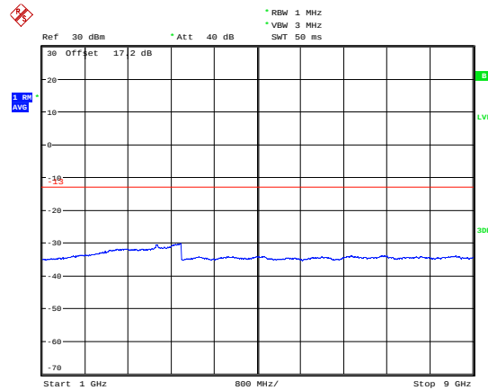
NB-IOT Band 5 CH-Low 1GHz-9GHz
