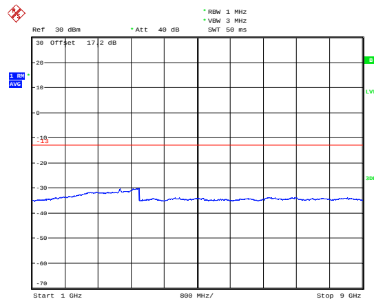
NB-IOT Band 5 CH-Middle 1GHz-9GHz
