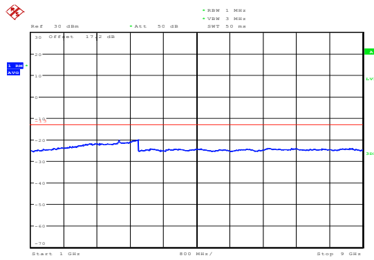
LTE Band 5 1.4MHz CH-High 1GHz ~9GHz
