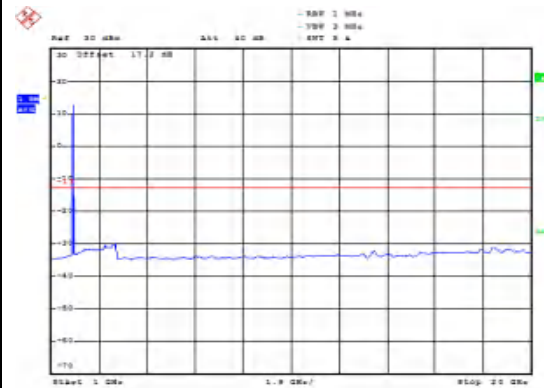
LTE Band 2 1.4MHz CH-Low 1GHz~20GHz
