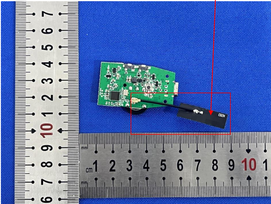
FPC Antenna
