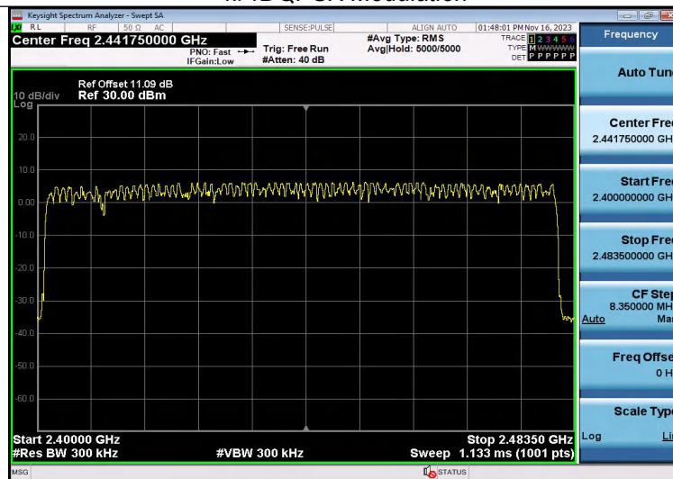
8DPSK Modulation
