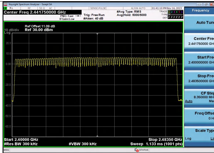
GFSK Modulation
