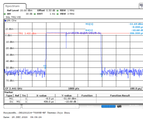
8DPSK_Hopping_3DH1
