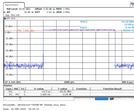
PI/4-DQPSK_Hopping_2DH3
