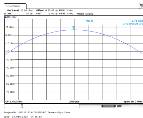
8DPSK_Low_3DH1
