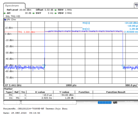
8DPSK_Hopping_3DH5
