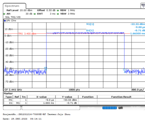
8DPSK_Hopping_3DH3
