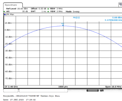
8DPSK_High_3DH1
