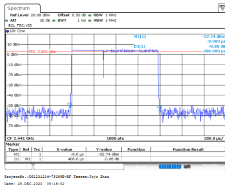
PI/4-DQPSK_Hopping_2DH1
