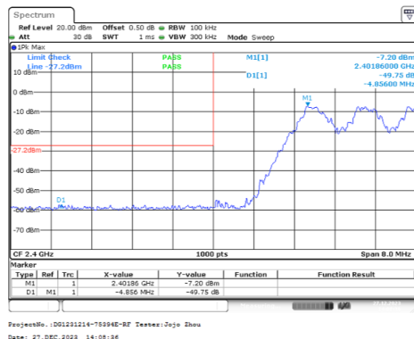
GFSK_Hopping_Lower_DH1
