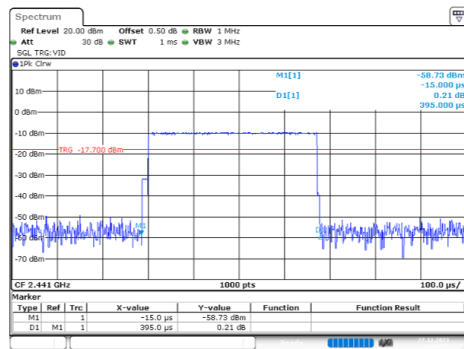
GFSK_Mid_DH1
