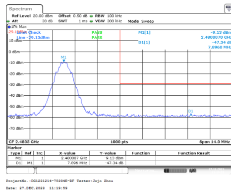
GFSK_High_DH1
