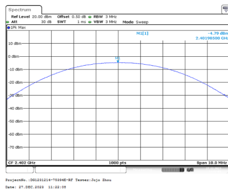
PI/4-DQPSK_Low_2DH1
