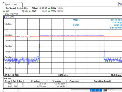
GFSK_Mid_DH3
