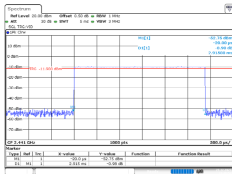
GFSK_Mid_DH5
