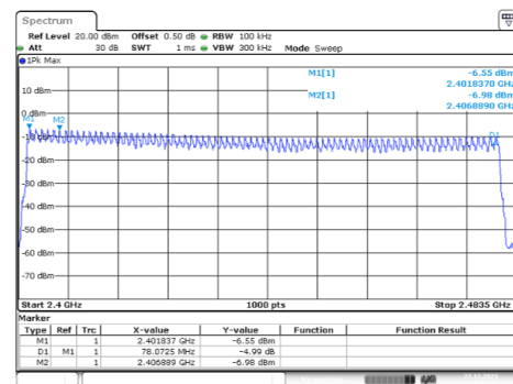
PI/4-DQPSK_Hopping_2DH1
