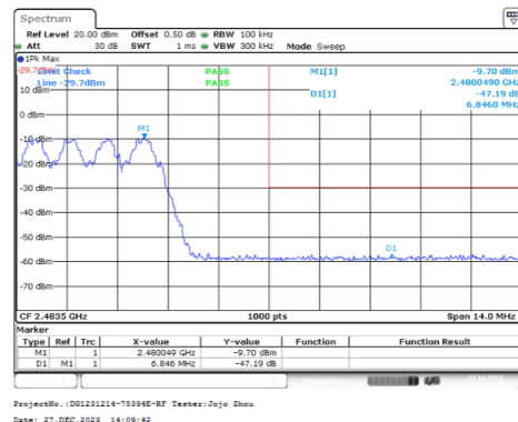
GFSK_Hopping_Upper_DH1
