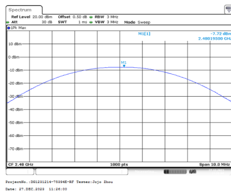
PI/4-DQPSK_High_2DH1
