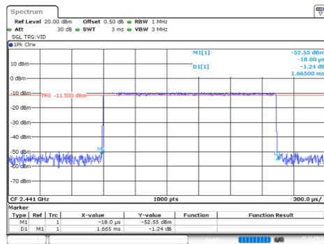
PI/4-DQPSK_Mid_2DH3
