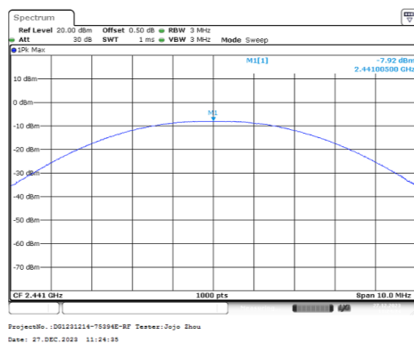
PI/4-DQPSK_Mid_2DH1
