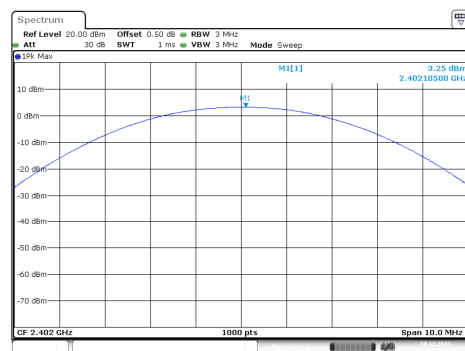
PI/4-DQPSK_Low_2DH1
