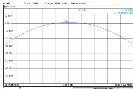
GFSK_High_DH1
