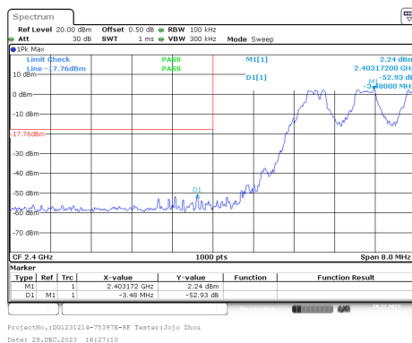
GFSK_Hopping_Lower_DH1
