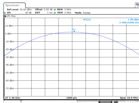
PI/4-DQPSK_High_2DH1
