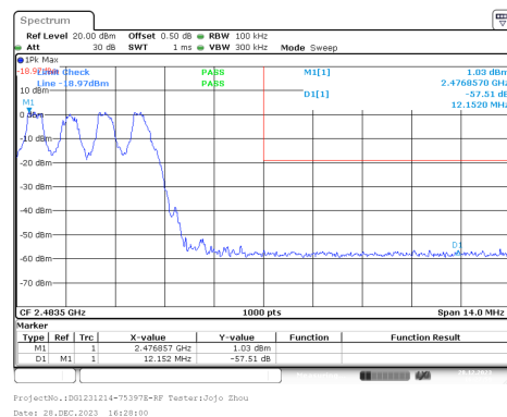
GFSK_Hopping_Upper_DH1
