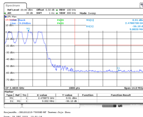
GFSK_Hopping_Upper_DH1
