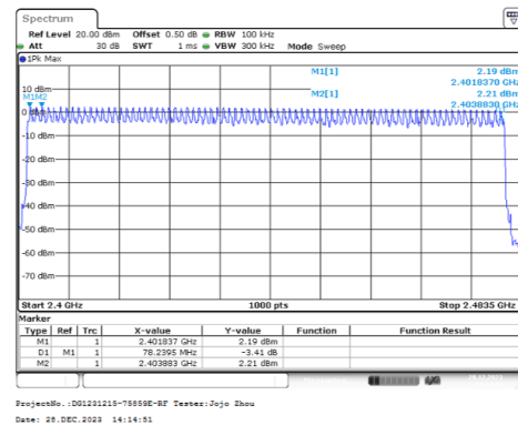
PI/4-DQPSK_Hopping_2DH1
