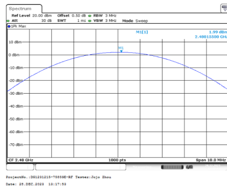
PI/4-DQPSK_High_2DH1
