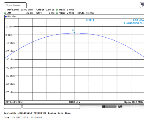
GFSK_Mid_DH1
