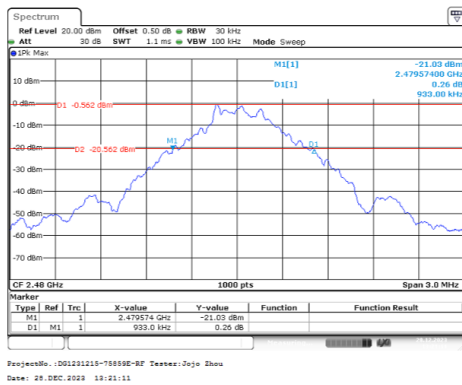
GFSK_High_DH1
