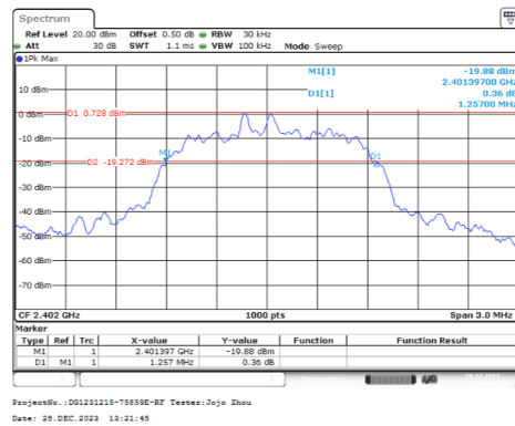
PI/4-DQPSK_Low_2DH1
