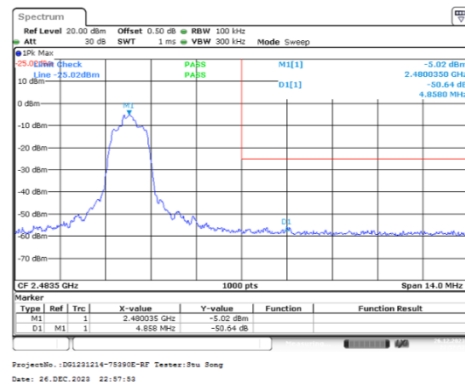
8DPSK_High_3DH1
