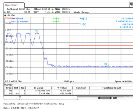
GFSK_Hopping_Upper_DH1
