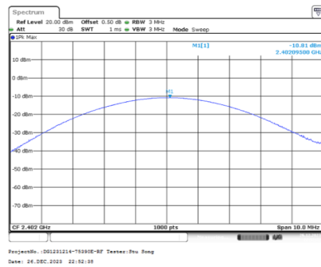
8DPSK_Low_3DH1
