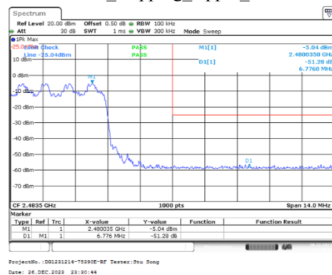
8DPSK_Hopping_Upper_3DH1
