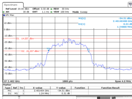
PI/4-DQPSK_Low_2DH1
