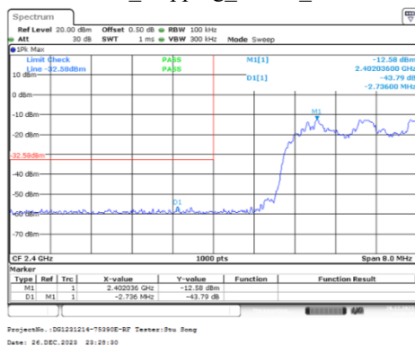
8DPSK_Hopping_Lower_3DH1
