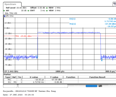
PI/4-DQPSK_Mid_2DH3
