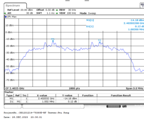
8DPSK_Low_3DH1
