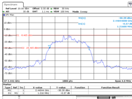
8DPSK_Mid_3DH1
