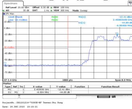
PI/4-DQPSK_Hopping_Lower_2DH1
