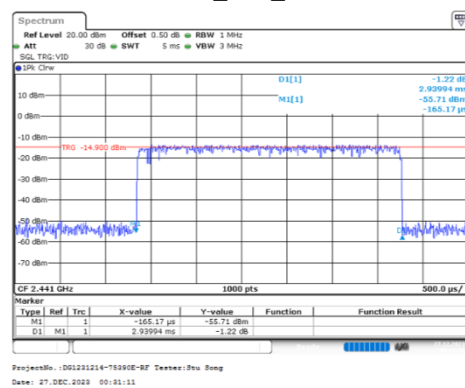
8DPSK_Mid_3DH5
