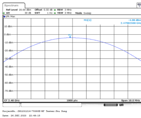
PI/4-DQPSK_High_2DH1
