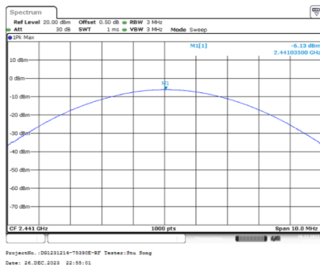
8DPSK_Mid_3DH1
