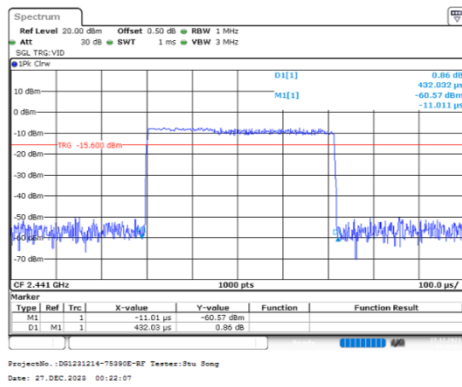
PI/4-DQPSK_Mid_2DH1
