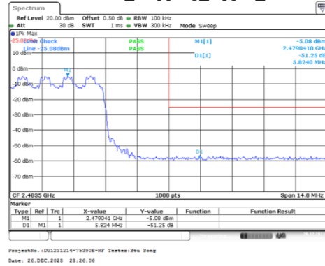
PI/4-DQPSK_Hopping_Upper_2DH1
