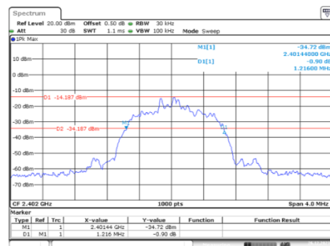
8DPSK_Low_3DH1
