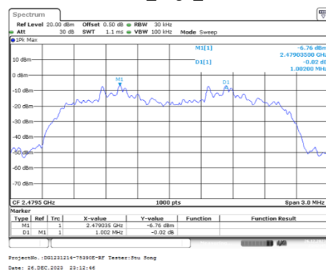
8DPSK_High_3DH1
