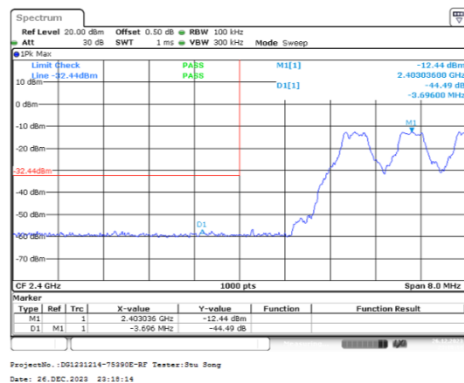
GFSK_Hopping_Lower_DH1
