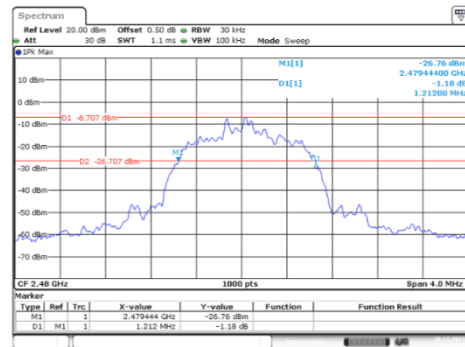
8DPSK_High_3DH1
