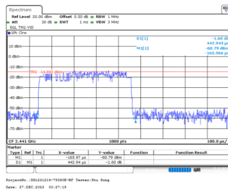
8DPSK_Mid_3DH1
