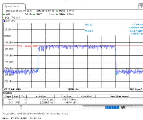
8DPSK_Mid_3DH3
