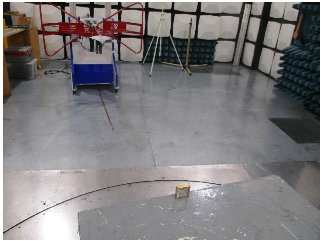
Test Setup – Radiated emission from 1 GHz to 18 GHz
