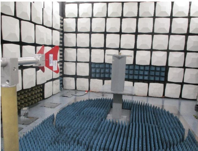
Test Setup – Radiated emission from 18 GHz to 25 GHz
