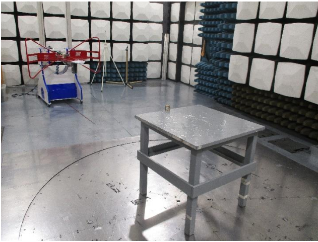
Test Setup – Radiated emission from 1 GHz to 18 GHz
