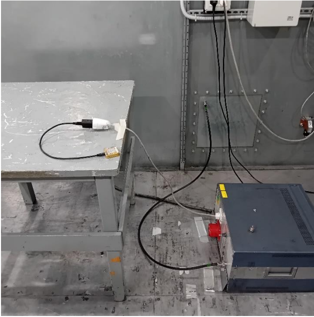
Test Setup – Measurement of disturbance voltage
