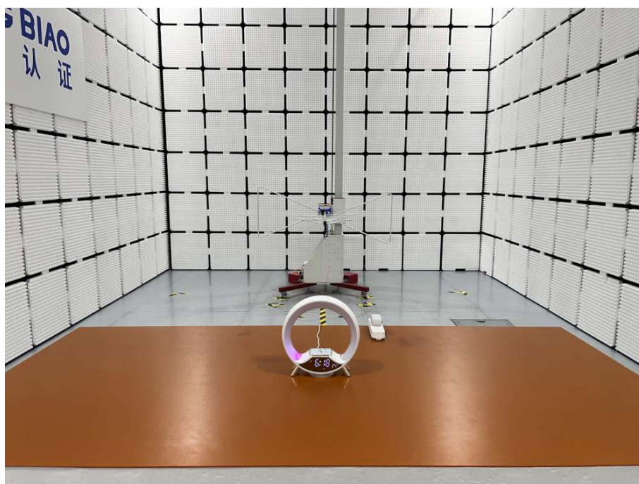
Radiated Emission Above 1GHz(BT)
