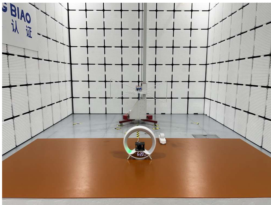
Radiated Emission Below 1GHz(Wireless Charging)
