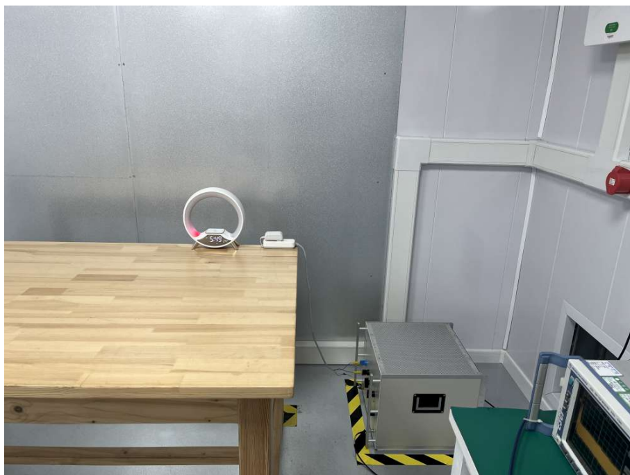
Conducted Emission(BT)
