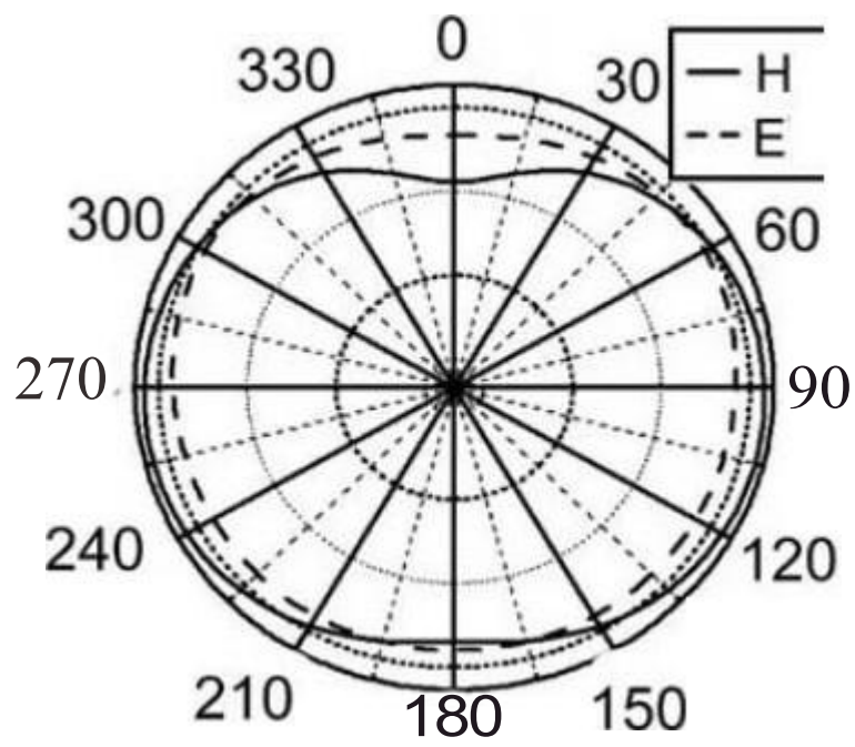
27.145/49.860 MHZ radiation pattern
