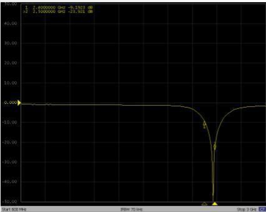
Return loss
