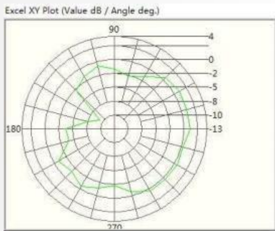
2D Radiation Pattern
