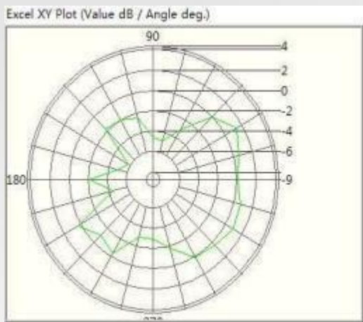
2D Radiation Pattern
