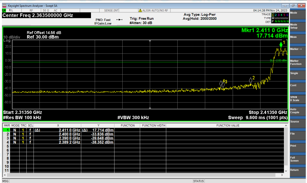
Band Edge(Hopping) NVNT 2409.5MHz Hopping Emission
