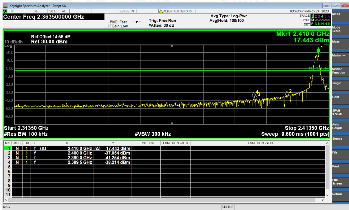
Band Edge NVNT 2409.5MHz No-Hopping Emission
