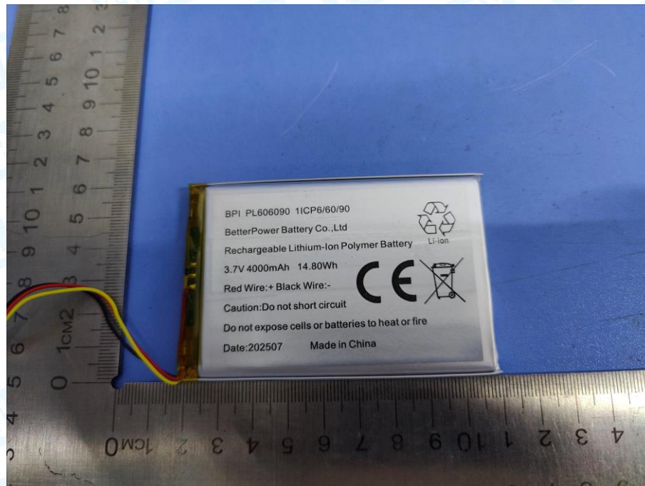
Photo 14 Battery Appearance
